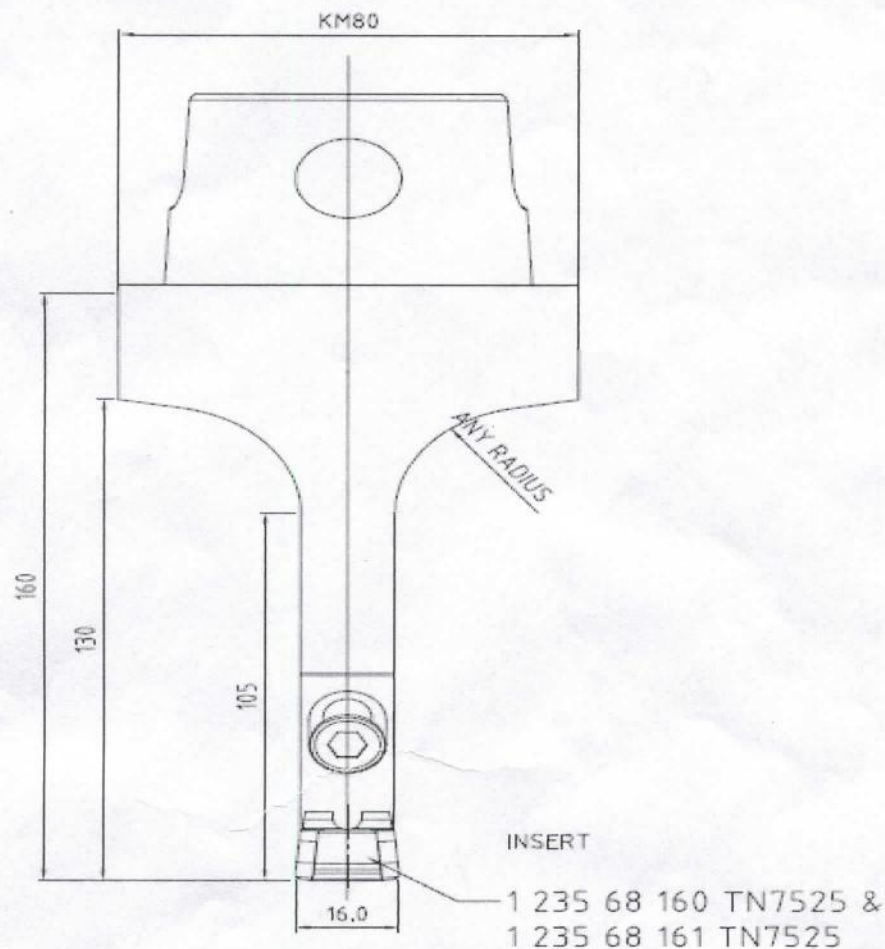
SCHEMATIC DRG 16MM TOOL
