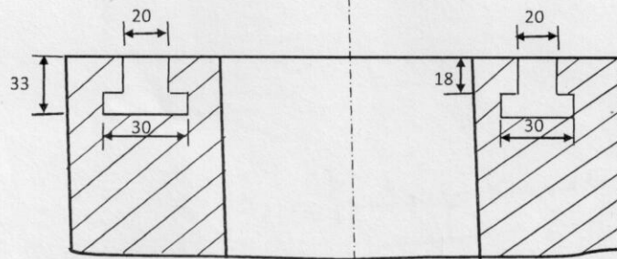
Section Z-Z
