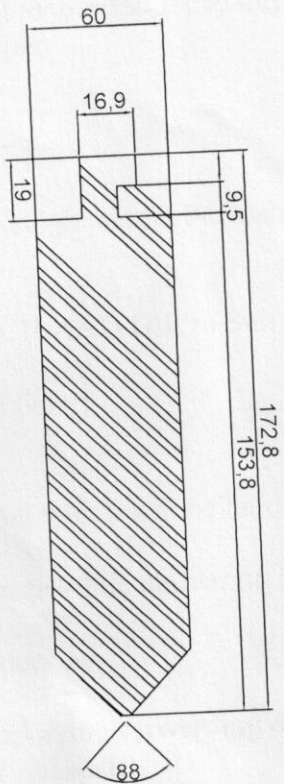
PUNCH SKETCH
