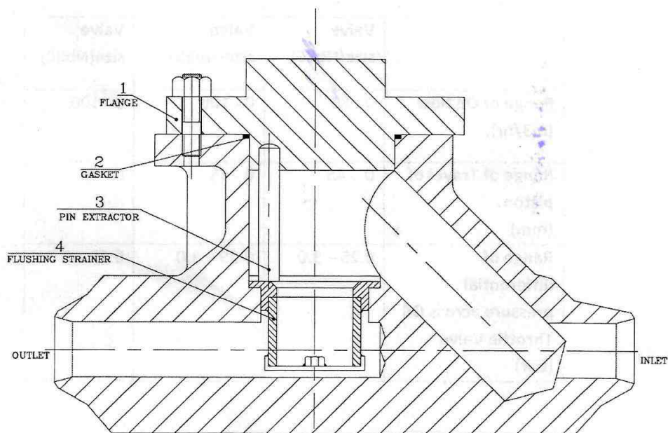
Flushing Operation (Figure-2)
