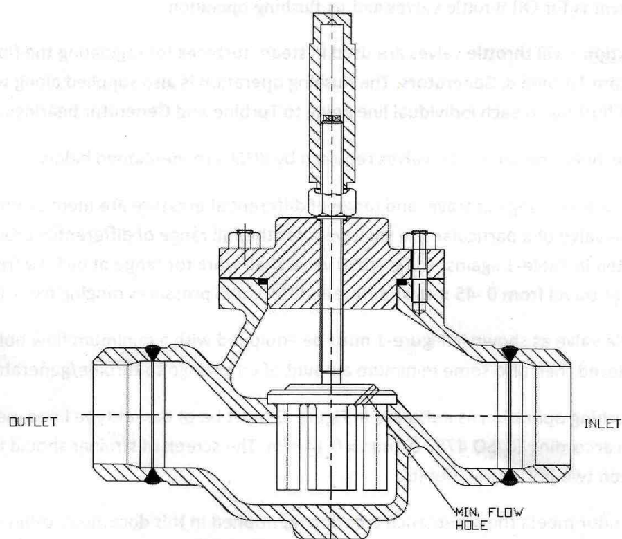
Oil Throttle valve (Figure-1)
