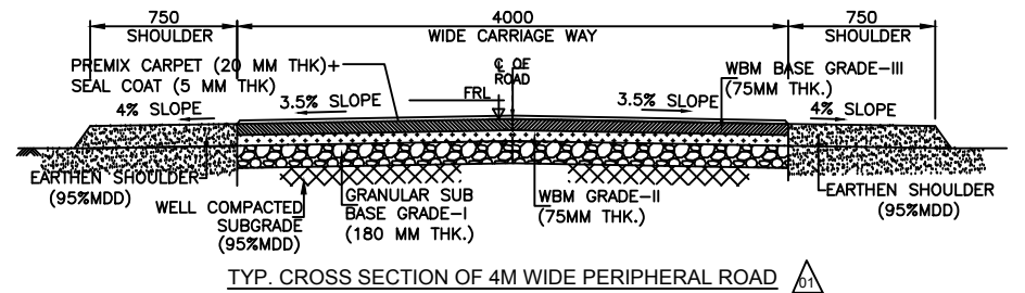
TYP. CROSS SECTION OF 4M WIDE PERIPHERAL ROAD
