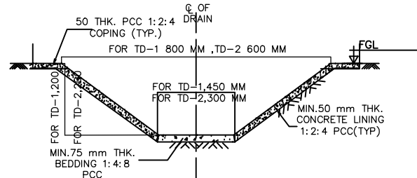
TYP. CROSS SECTION OF INTERNAL DRAINS
