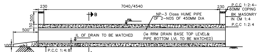
LONGITUDINAL SECTION OF PIPE CULVERT
