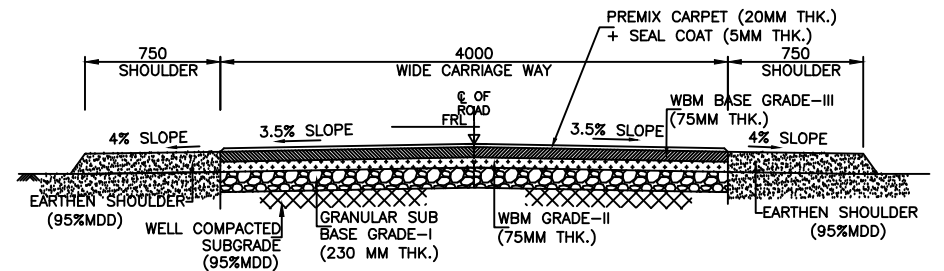
TYP. CROSS SECTION OF 4M WIDE APPROACH ROAD
