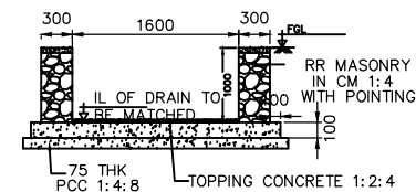
TYP. CROSS SECTION OF CATCH PIT
