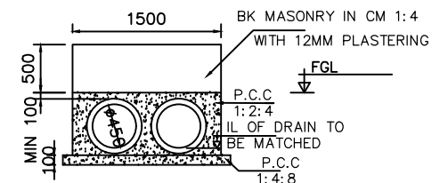
SECTION B-B FOR (PC-2,3,4)
