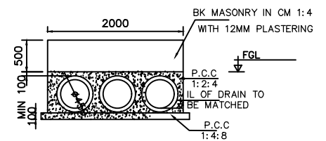
SECTION B-B FOR (PC-1)
