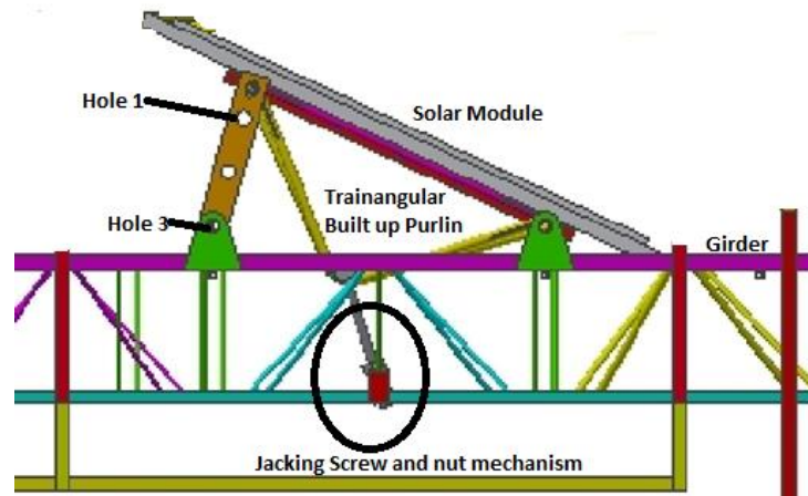
Fig-1: Schematic representation of 12 No. of Modules mounting on a purlin
