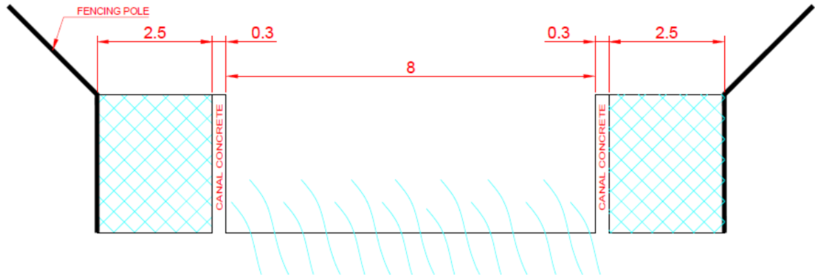
Fig-7: Cross Sectional View of the Canal at plant.
