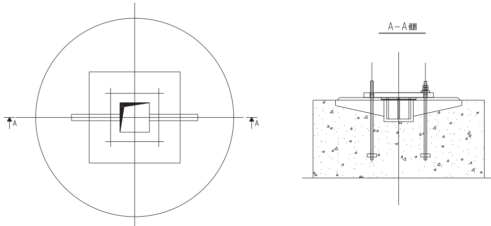
Schematic for embedments on the top of concrete column
