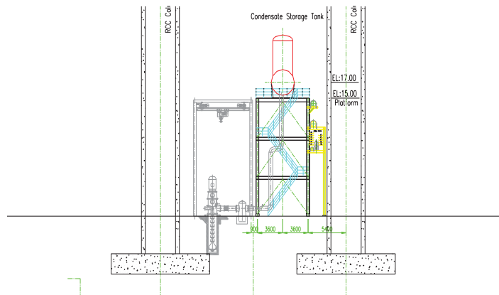
Condensate tank including deaerator
