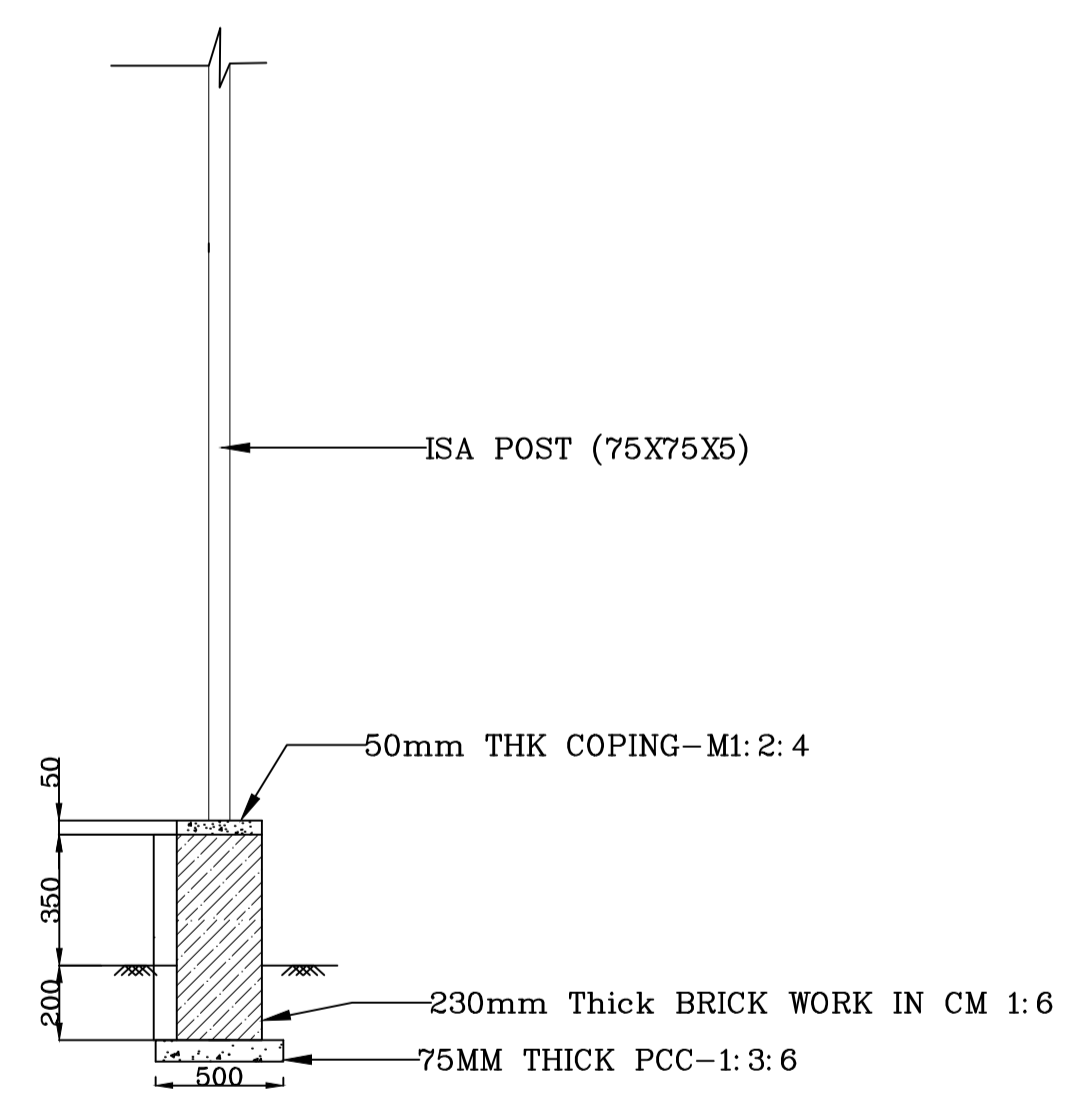
SECTION AT TOE-WALL
