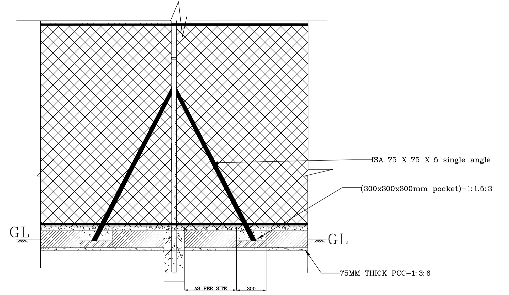
(TYP) SECTIONAL ELEVATION at CORNER
