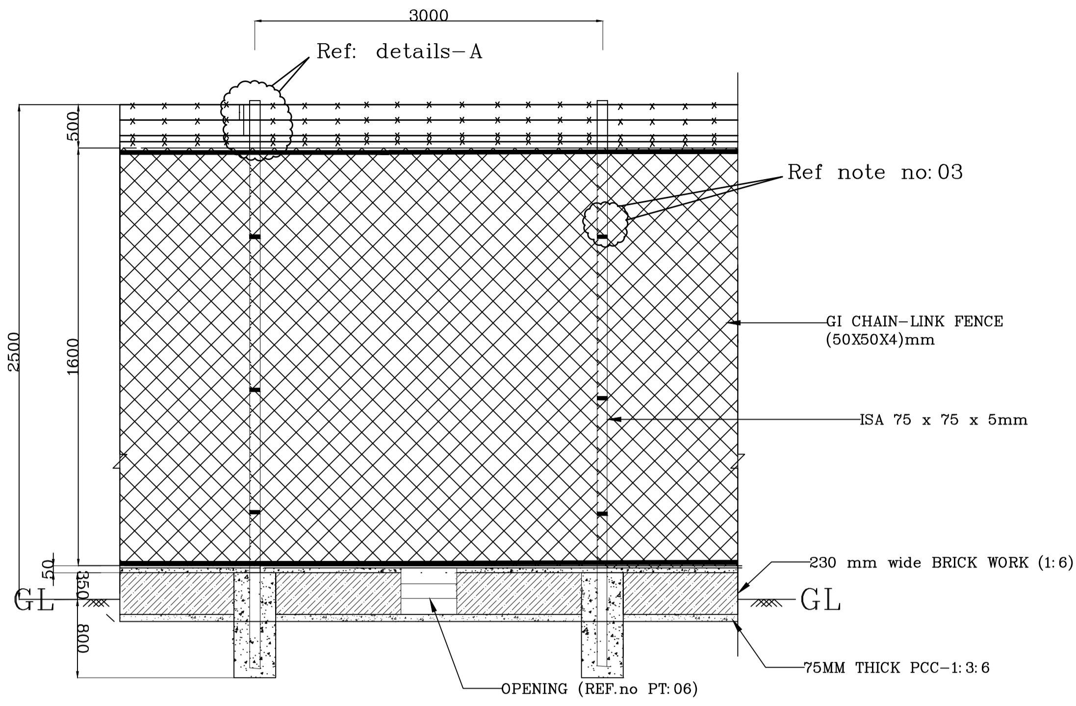
(TYP) SECTIONAL ELEVATION
