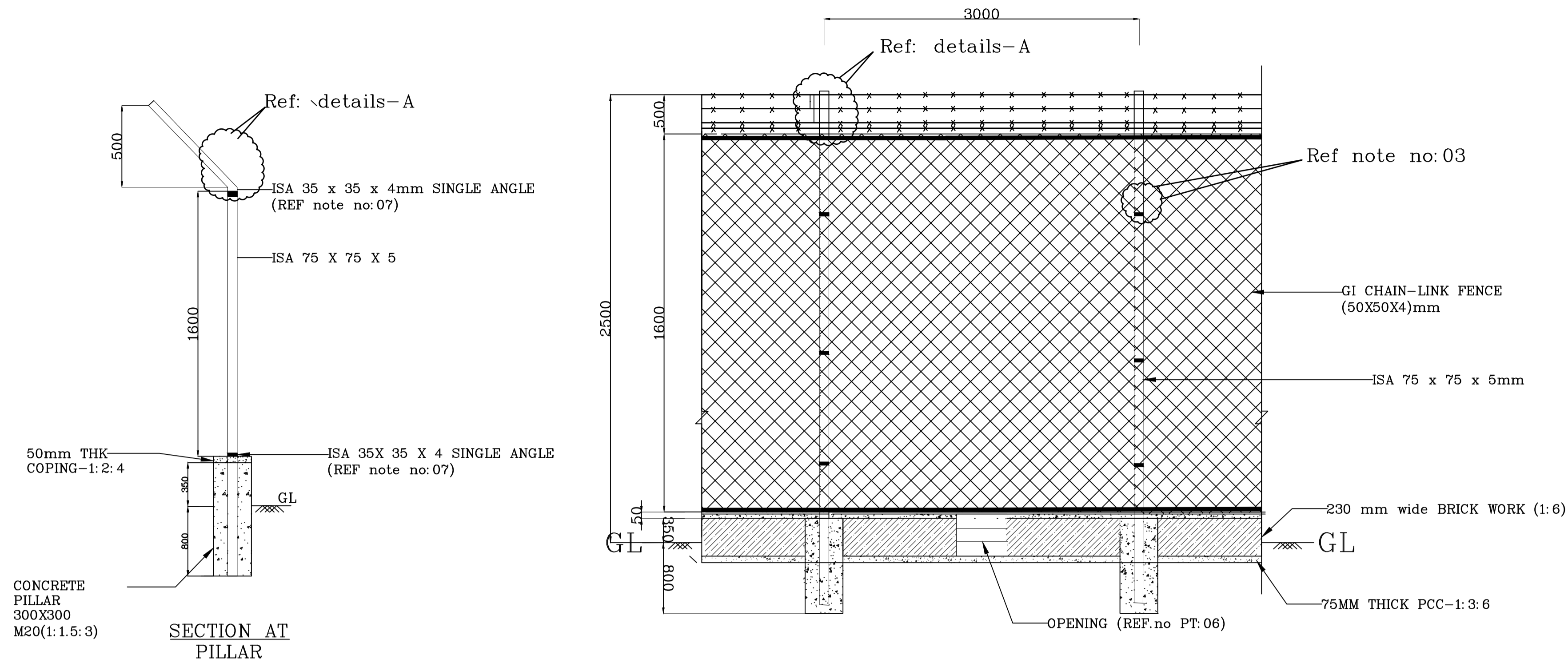
(TYP) SECTIONAL ELEVATION
