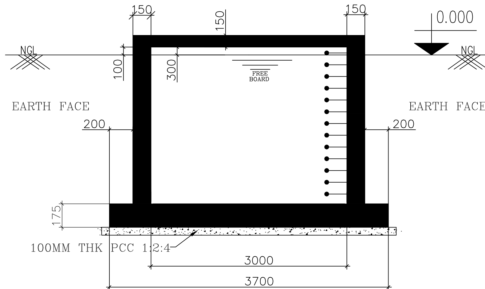
SECTION B-B
