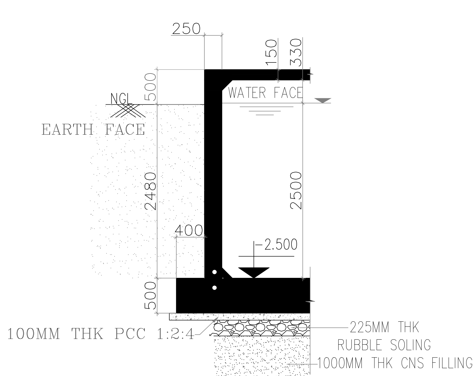
CONCRETE DIMENSION WALL-1&2 DETAILS
