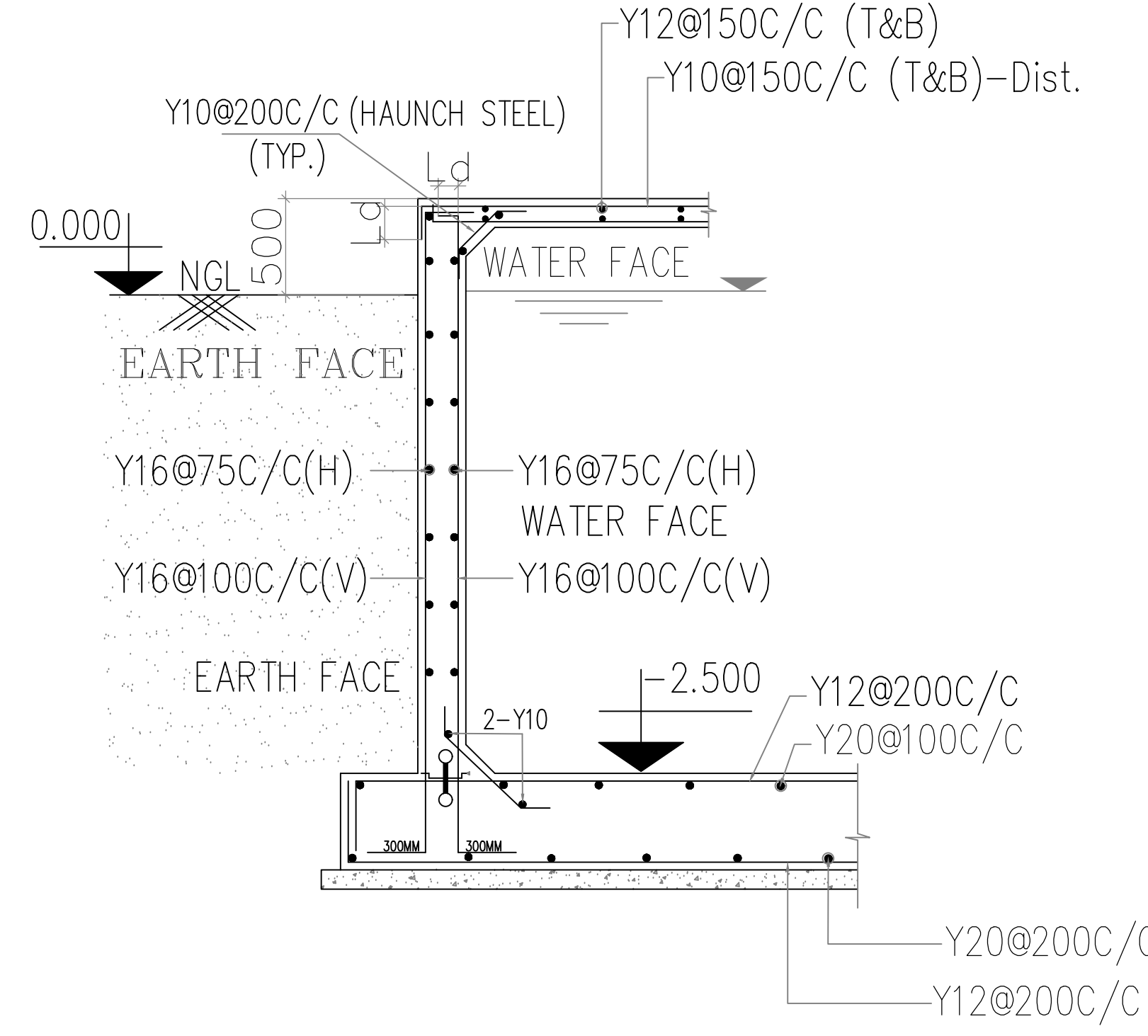
WALL-2 DETAIL SEC-DD REINFORCEMENT DETAIL
