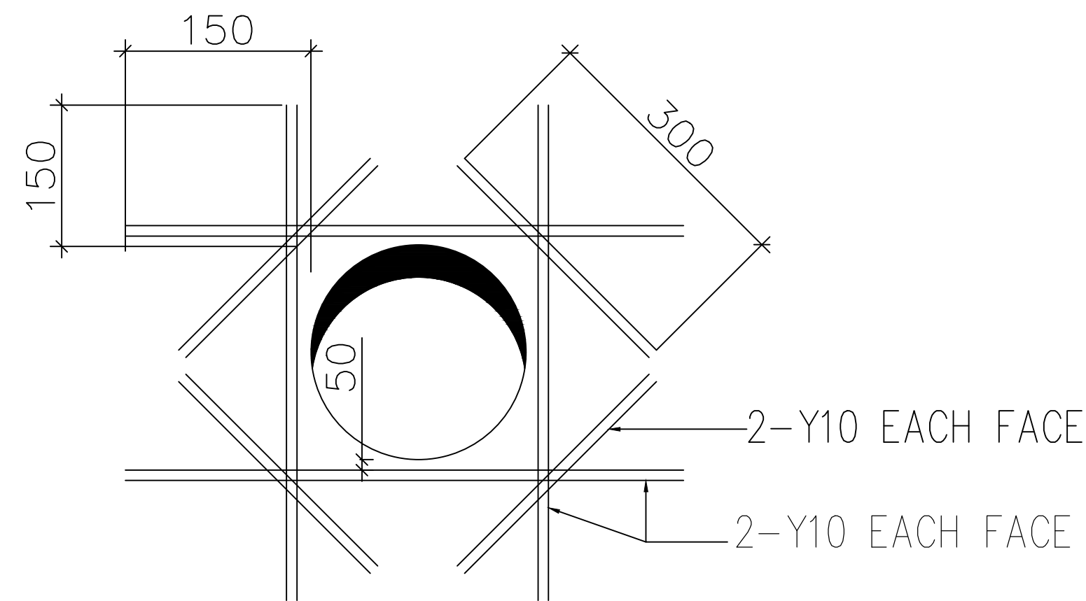
WALL-1 DETAIL SEC-CC REINFORCEMENT DETAIL
