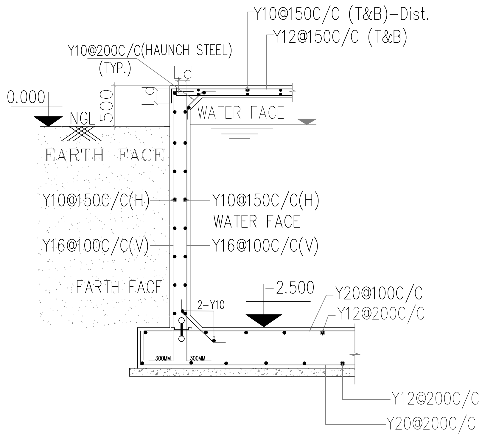
WALL-1 DETAIL SEC-CC REINFORCEMENT DETAIL
