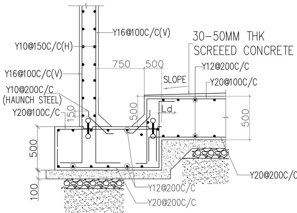
SILT PIT DETAIL SECTION E-E
