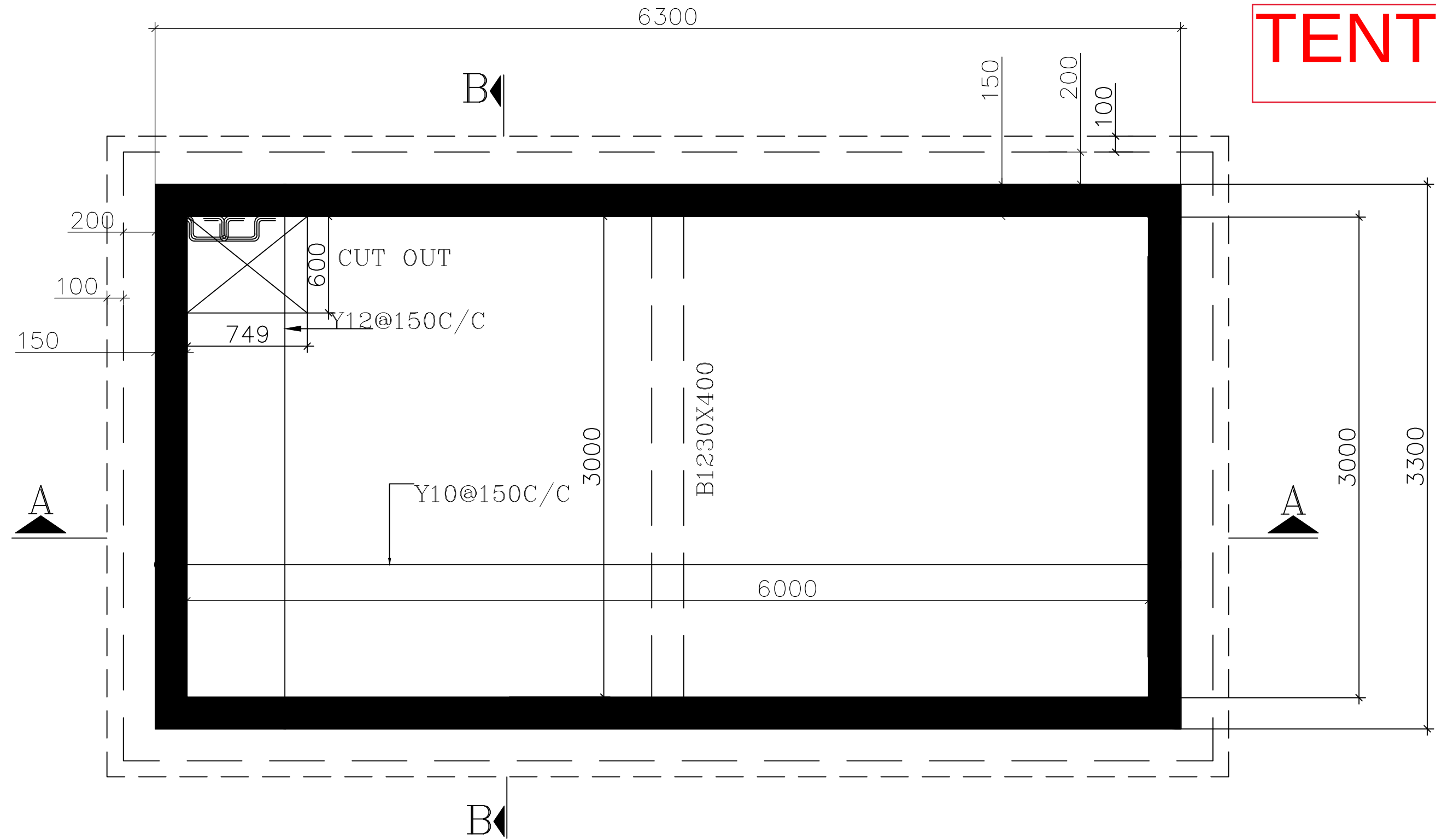
TOP SLAB PLAN @ +0.250 LVL (TOC)
