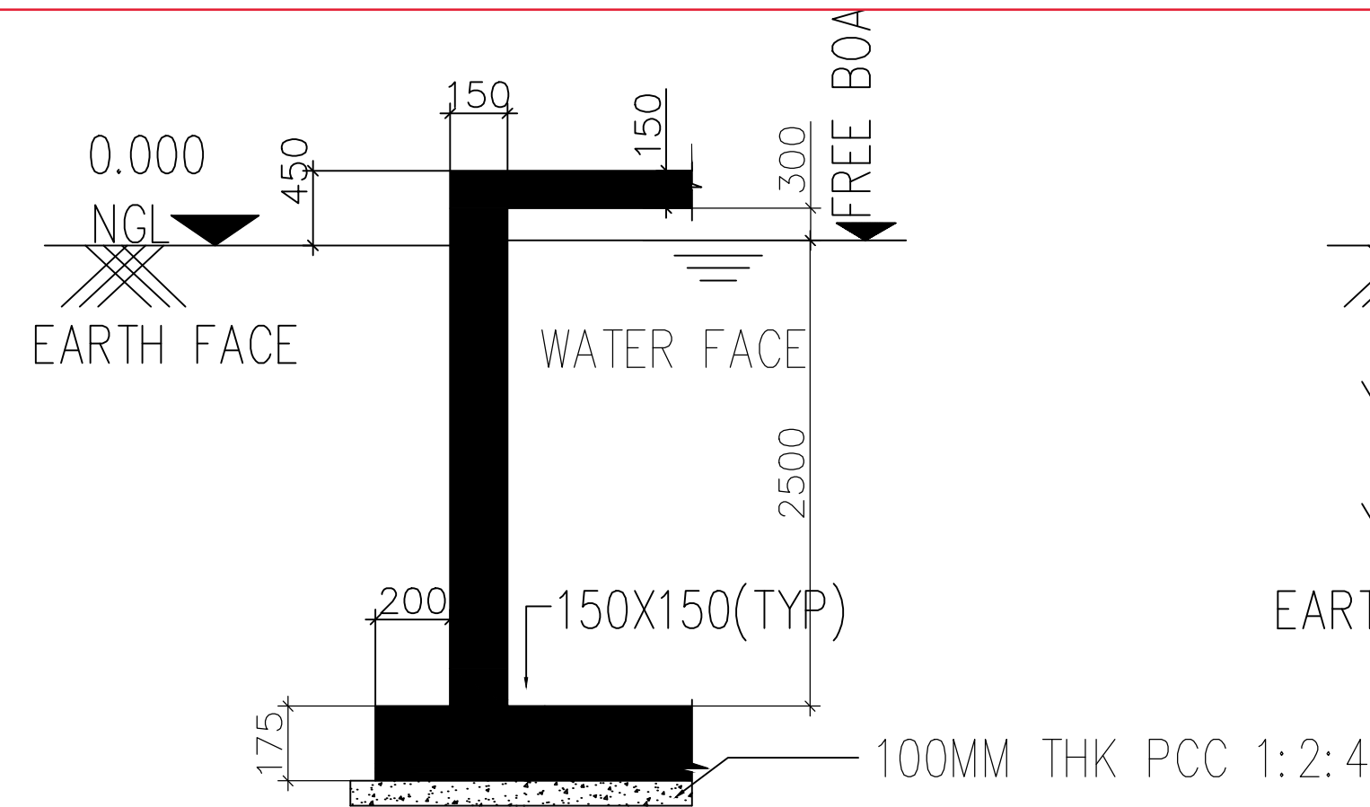
CONCRETE DIMENSION WALL-1&2 DETAILS
