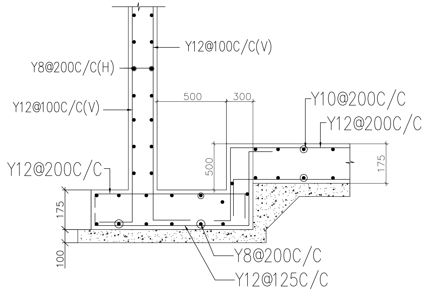
SILT PIT DETAIL SECTION E-E
