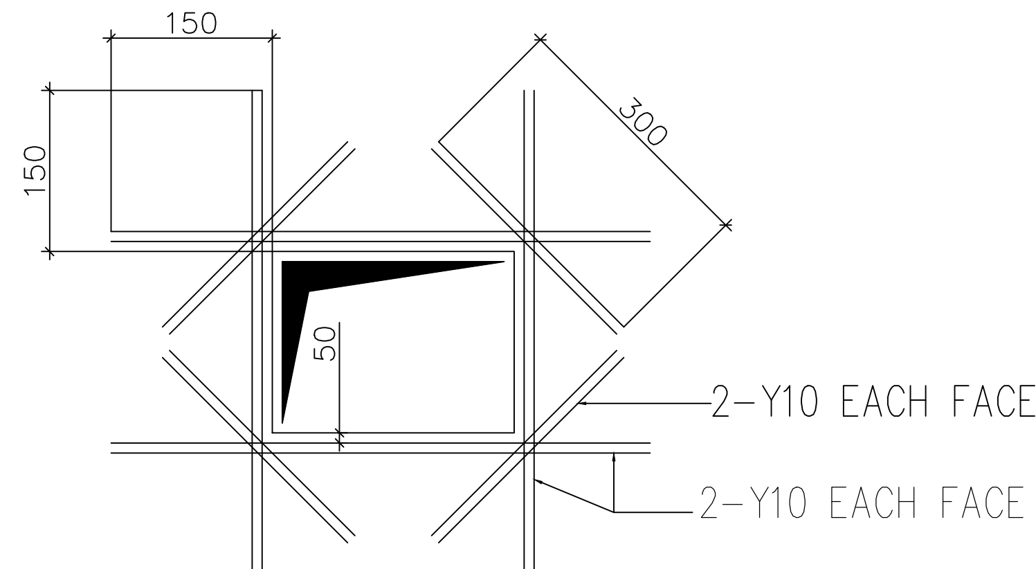
CONCRETE DIMENSION WALL-1&2 DETAILS
