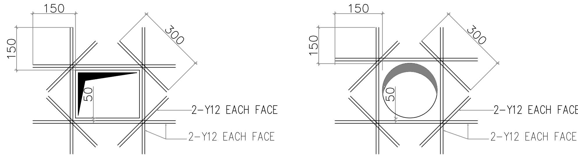
TYPICAL OPENING DETAIL
