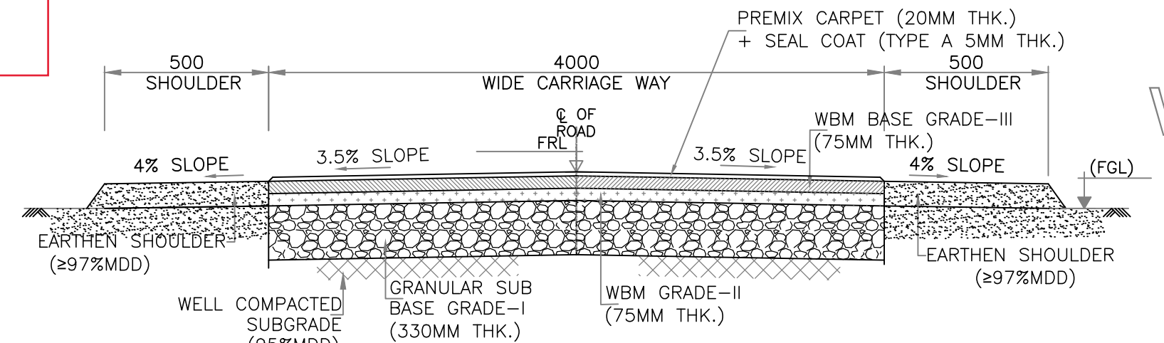
TYP. CROSS SECTION OF 4M WIDE APPROACH ROAD
