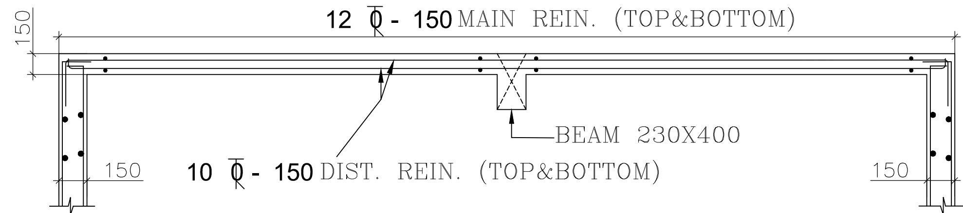
C/S OF ROOF SLAB(150MM THK) DETAIL
