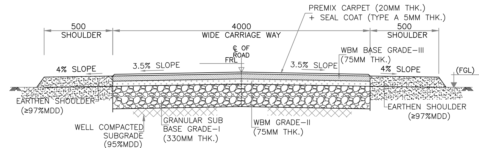
TYP. CROSS SECTION OF 4M WIDE PERIPHERAL ROAD
