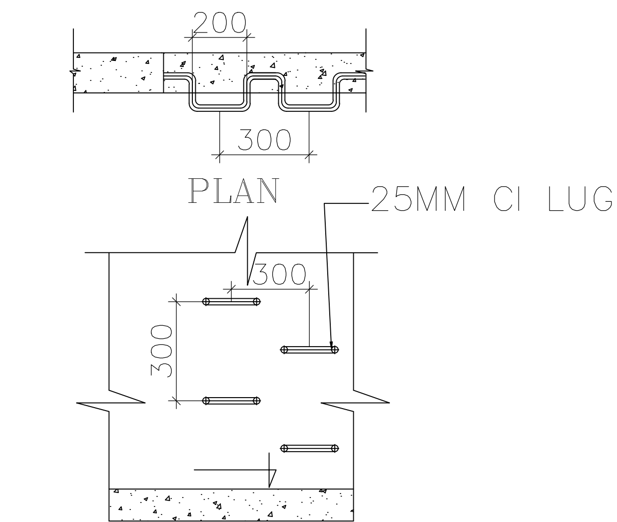
ELEVATION LADDER RUNGS DETAIL
