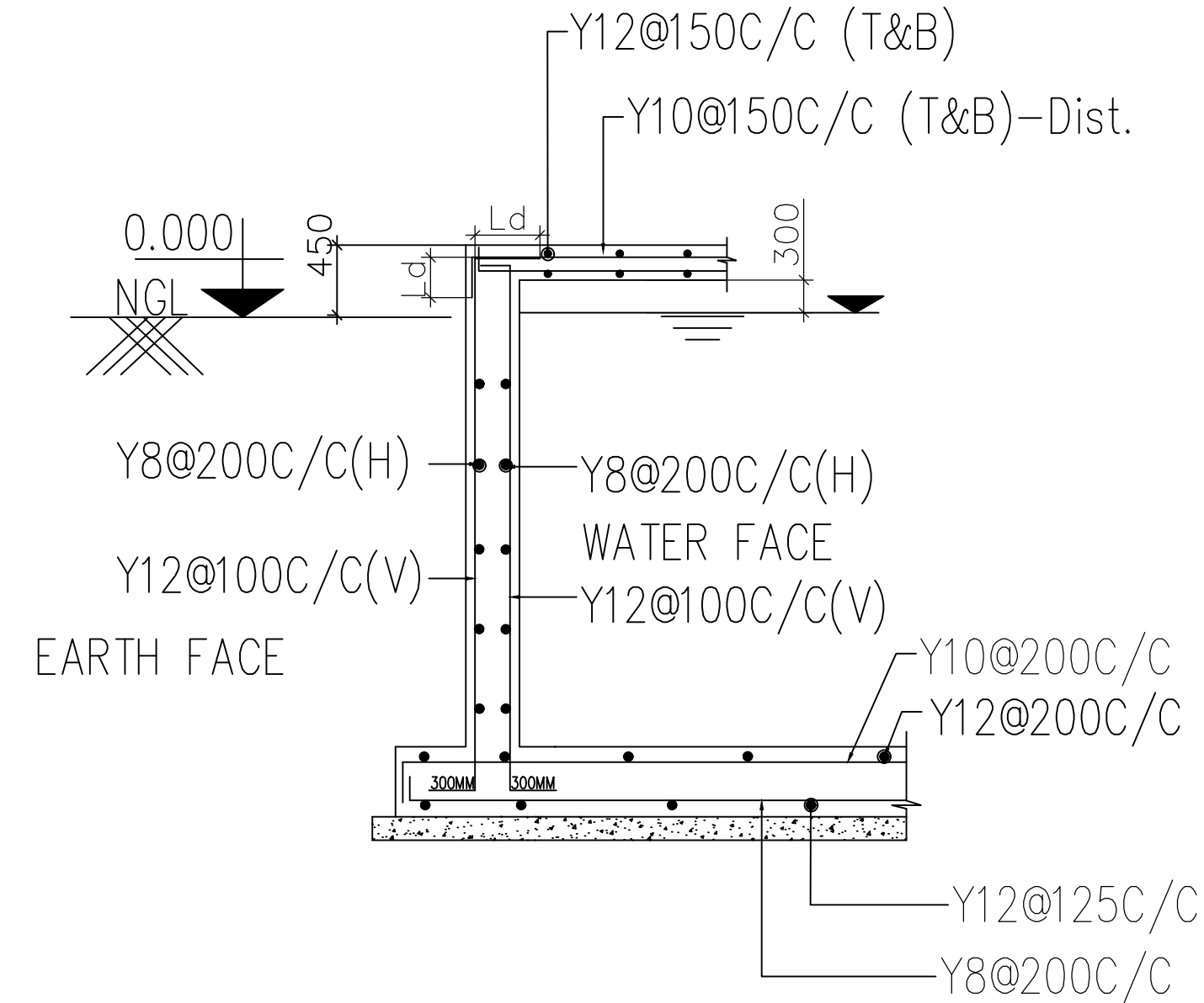
WALL-2 DETAIL SEC-DD REINFORCEMENT DETAIL
