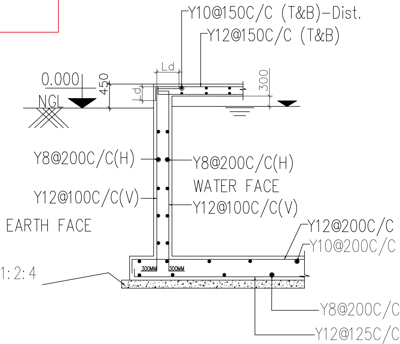
WALL-1 DETAIL SEC-CC REINFORCEMENT DETAIL
