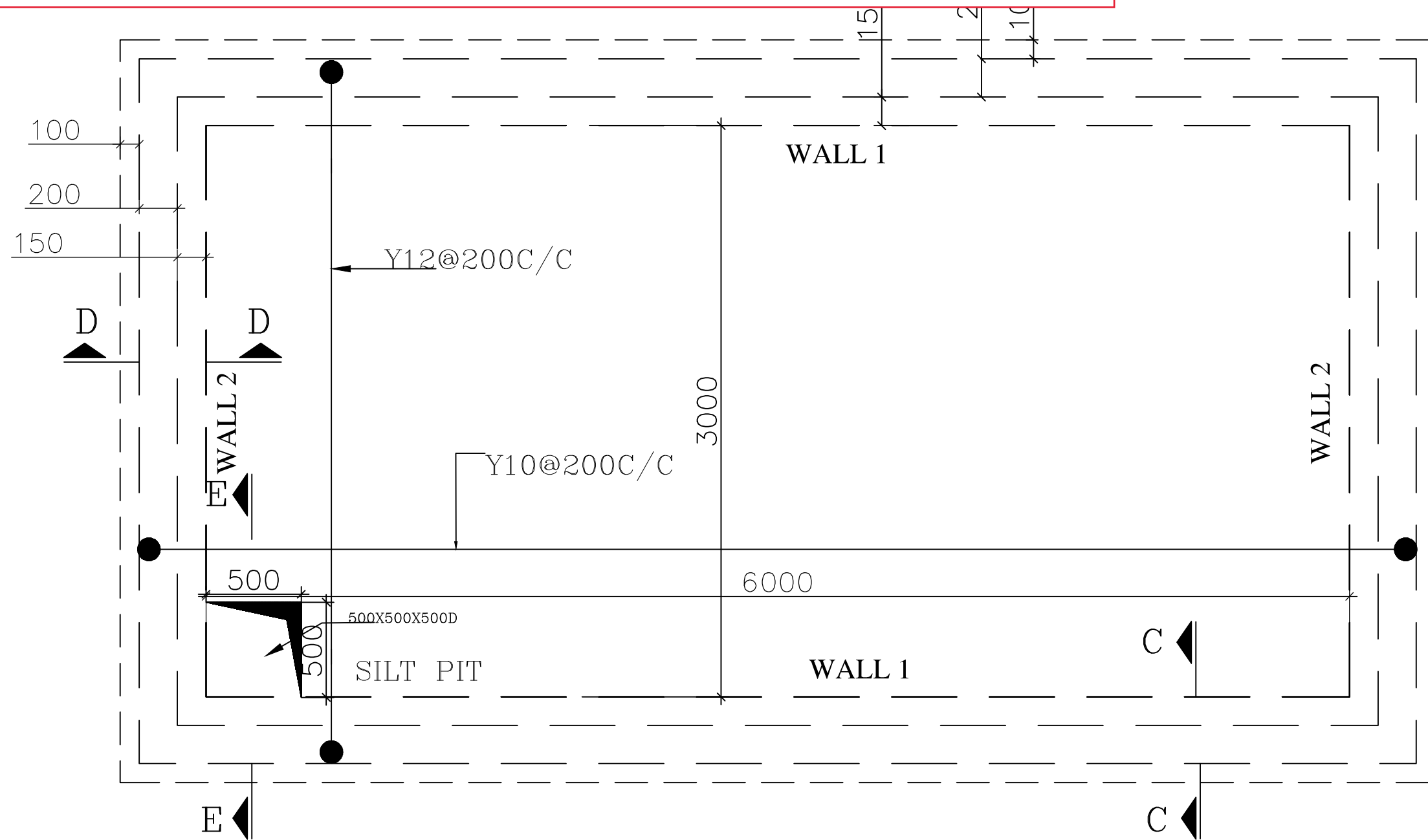
BASE SLAB TOP REINFORCEMENT DETAILS
