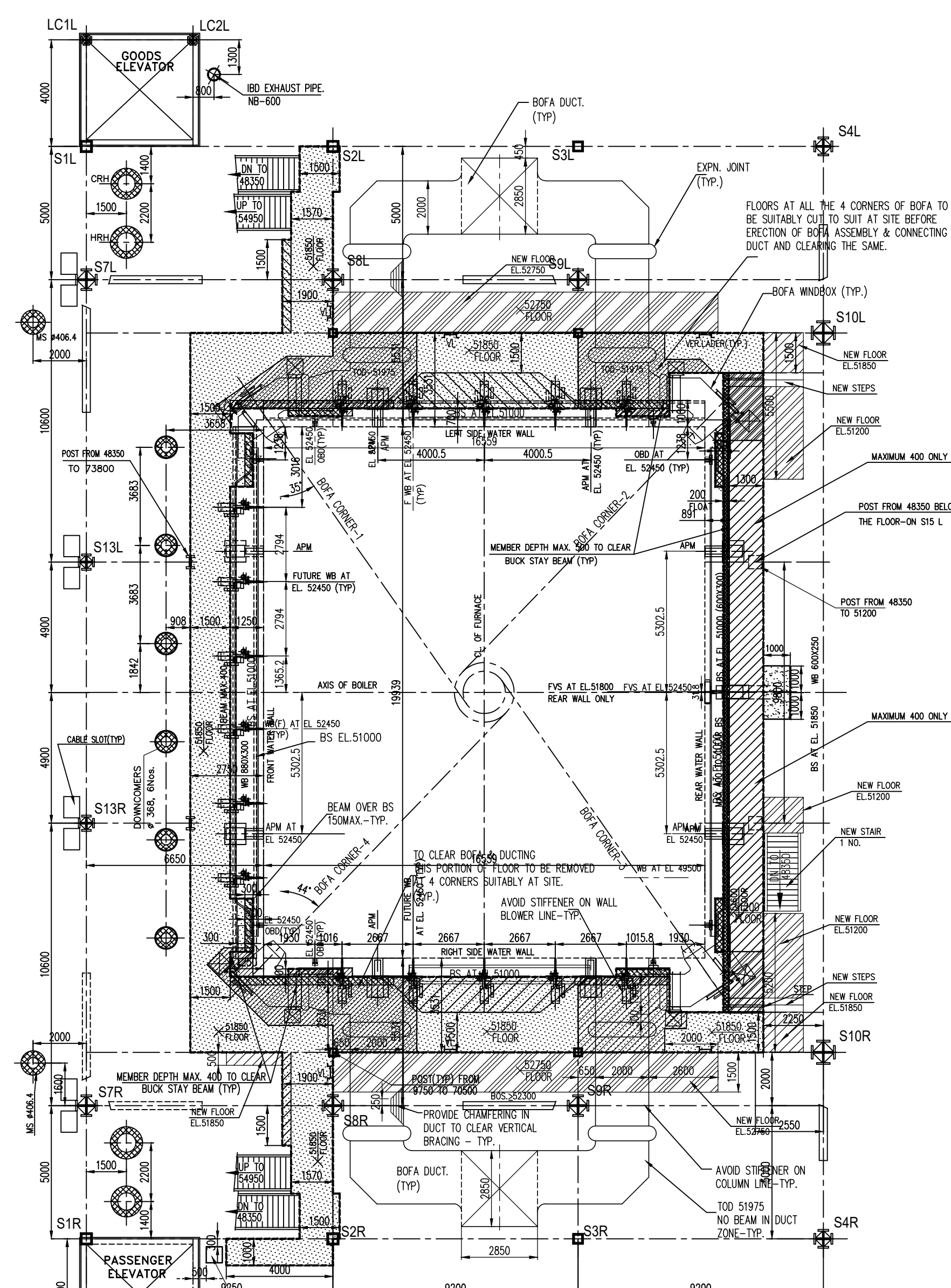
FLOOR PLAN AT EL 51850 (BOFA DUCTING WITH EXISTING & ADDITIONAL FLOOR ARRANGEMENT)
