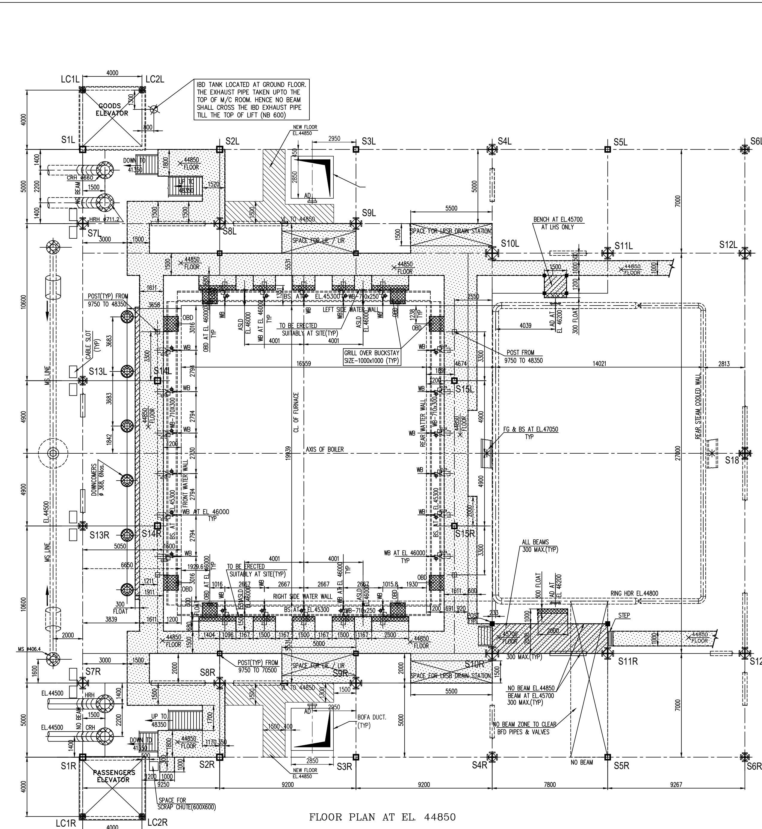
FLOOR PLAN AT EL 44850 (BOFA DUCTING WITH EXISTING & ADDITIONAL FLOOR ARRANGEMENT)
