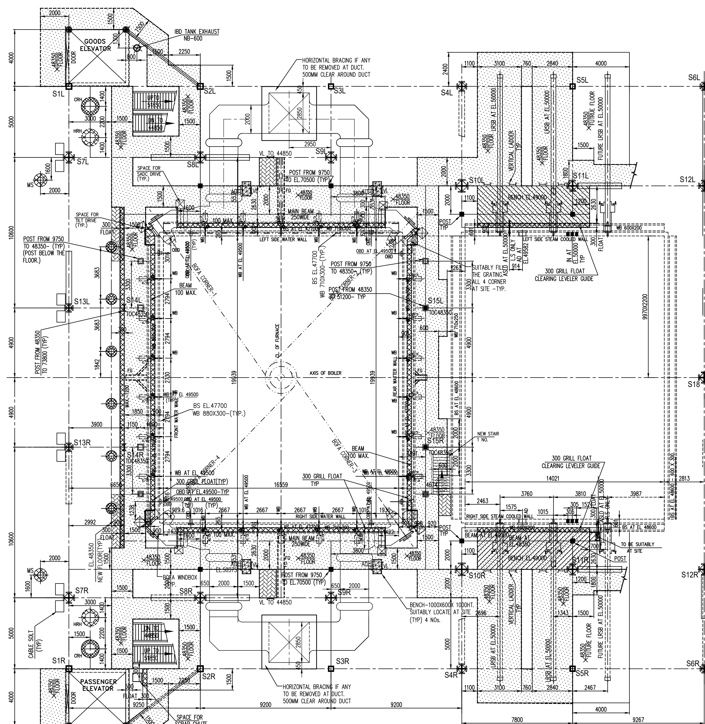
FLOOR PLAN AT EL 48350 (MBL-4) (BOFA DUCTING WITH EXISTING & ADDITIONAL FLOOR ARRANGEMENT)
