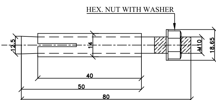
HEX BOLT
