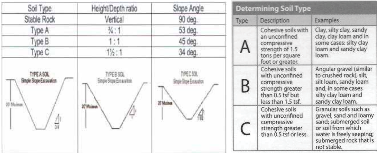
Fig. 13.2.2.1 Excavation Reference
