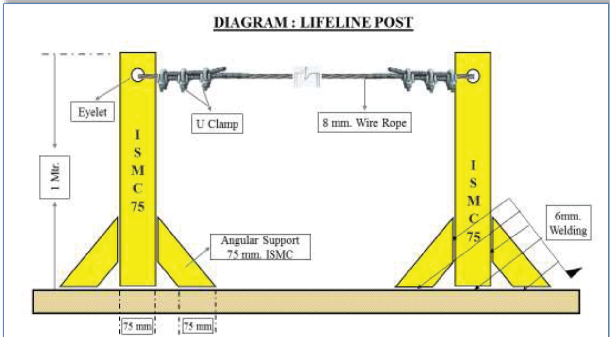
Fig. 13.2.1.1 Lifeline Post
