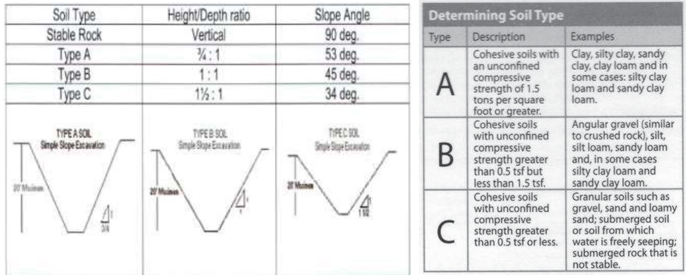
Fig. 13.2.2.1 Excavation Reference
