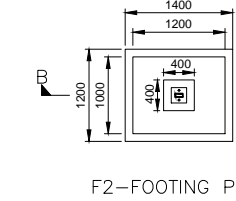
F2-FOOTING PLAN
