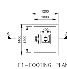
F1-FOOTING PLAN
