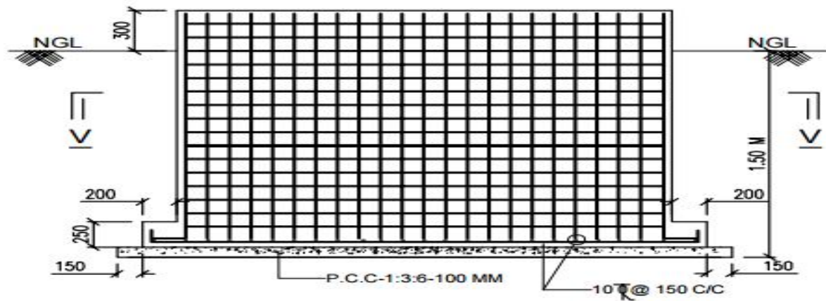
SECTION Z-Z
