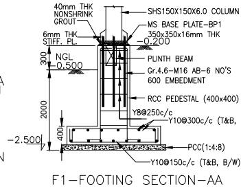
F1-FOOTING SECTION-AA
