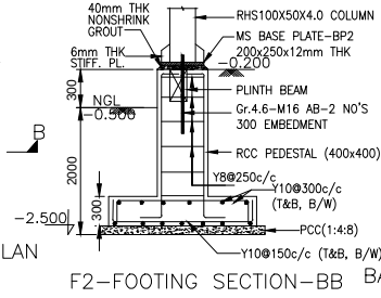
F2-FOOTING SECTION-BB
