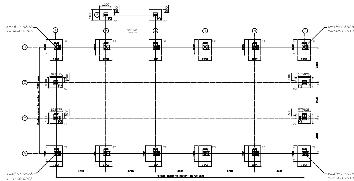
FOOTING LAYOUT
