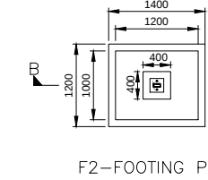
F2-FOOTING PLAN
