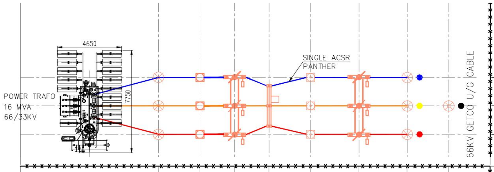
Tentative Switch yard plan
