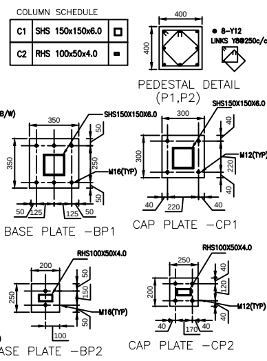
BASE PLATE -BP2
