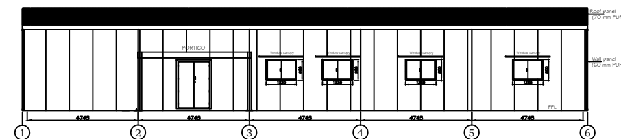
SIDE WALL PANEL ELEVATION IN LINE D
