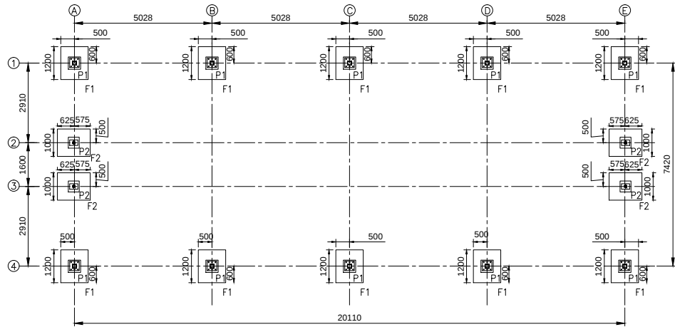
FOOTING LAYOUT
