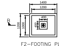
F2-FOOTING PLAN
