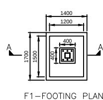
F1-FOOTING PLAN
