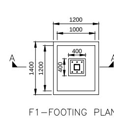
F1-FOOTING PLAN
