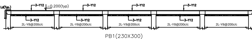
PLINTH BEAM LAYOUT
