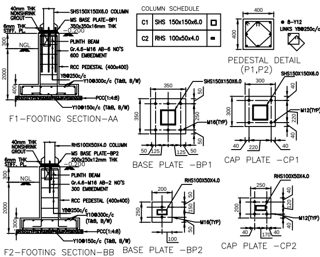
F2-FOOTING SECTION-BB
