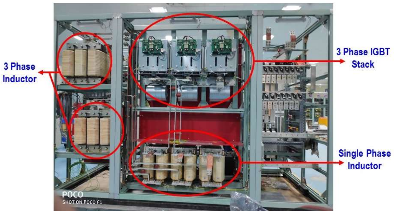
Rear Internal View Of A 1.25MW PCU
