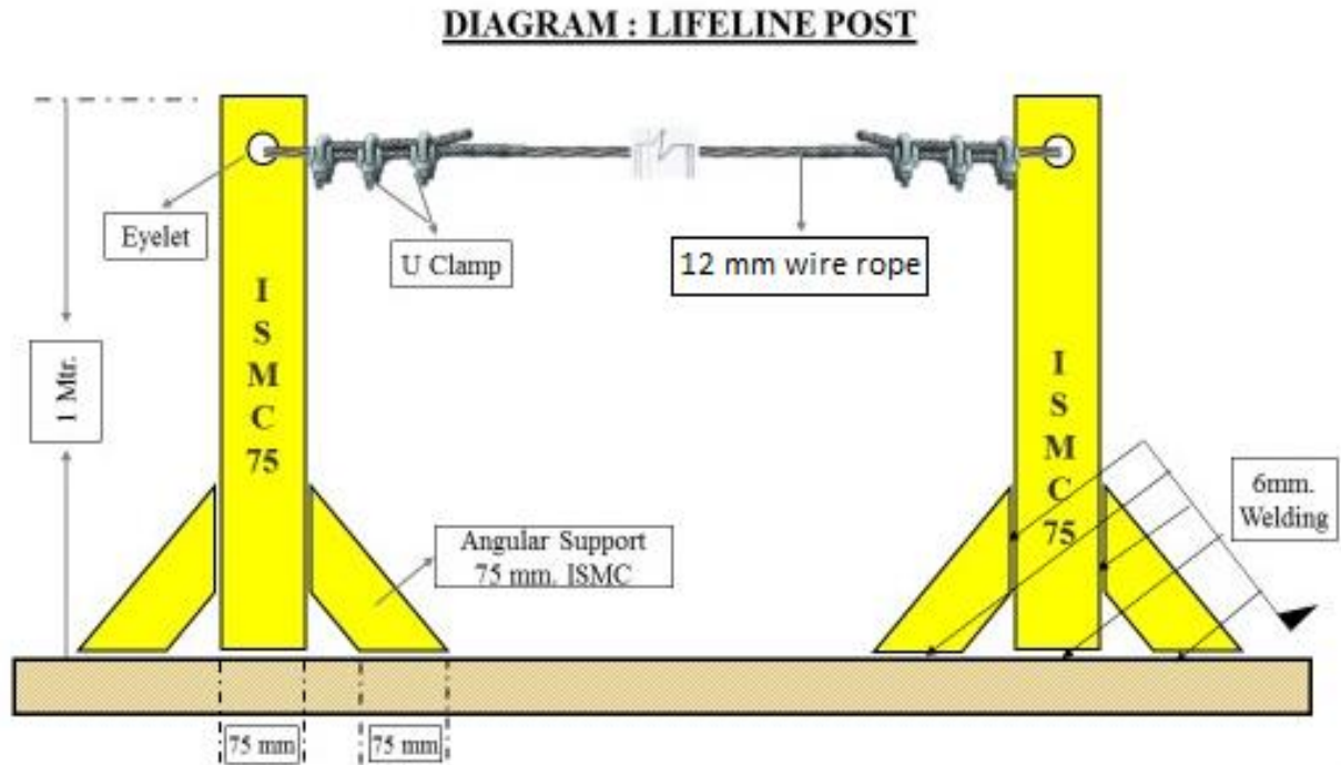
Fig. 13.2.1.1 Lifeline Post
