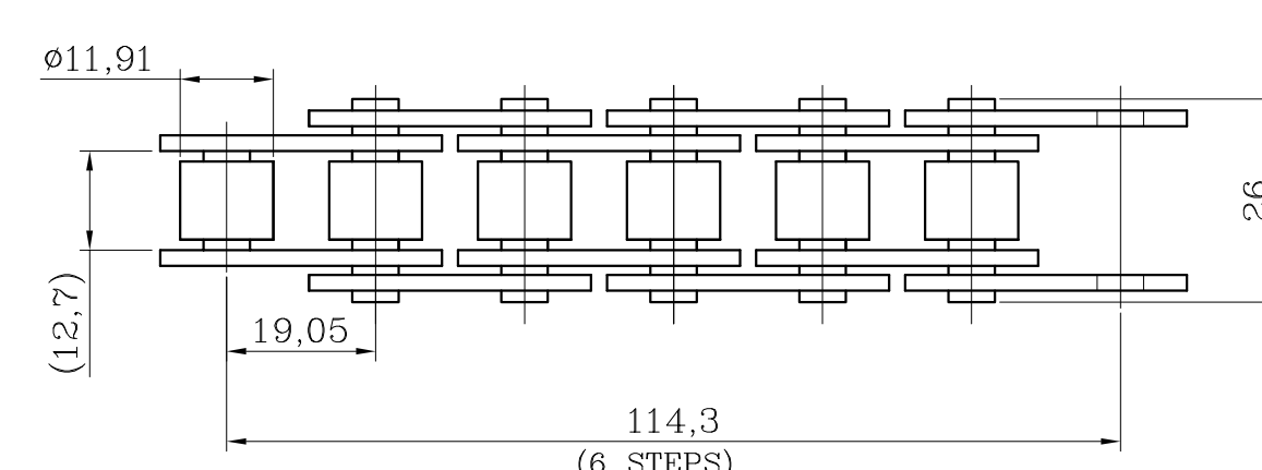
ITEM-4 CHAIN, ROLLER (6 LINKS)
