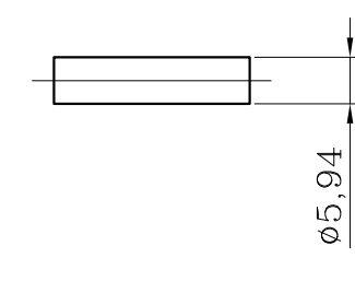
ITEM-8 PIN
