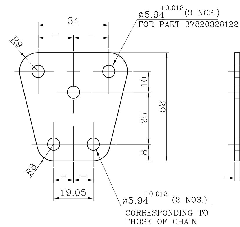
ITEM-10 LINK, CONNECTION
