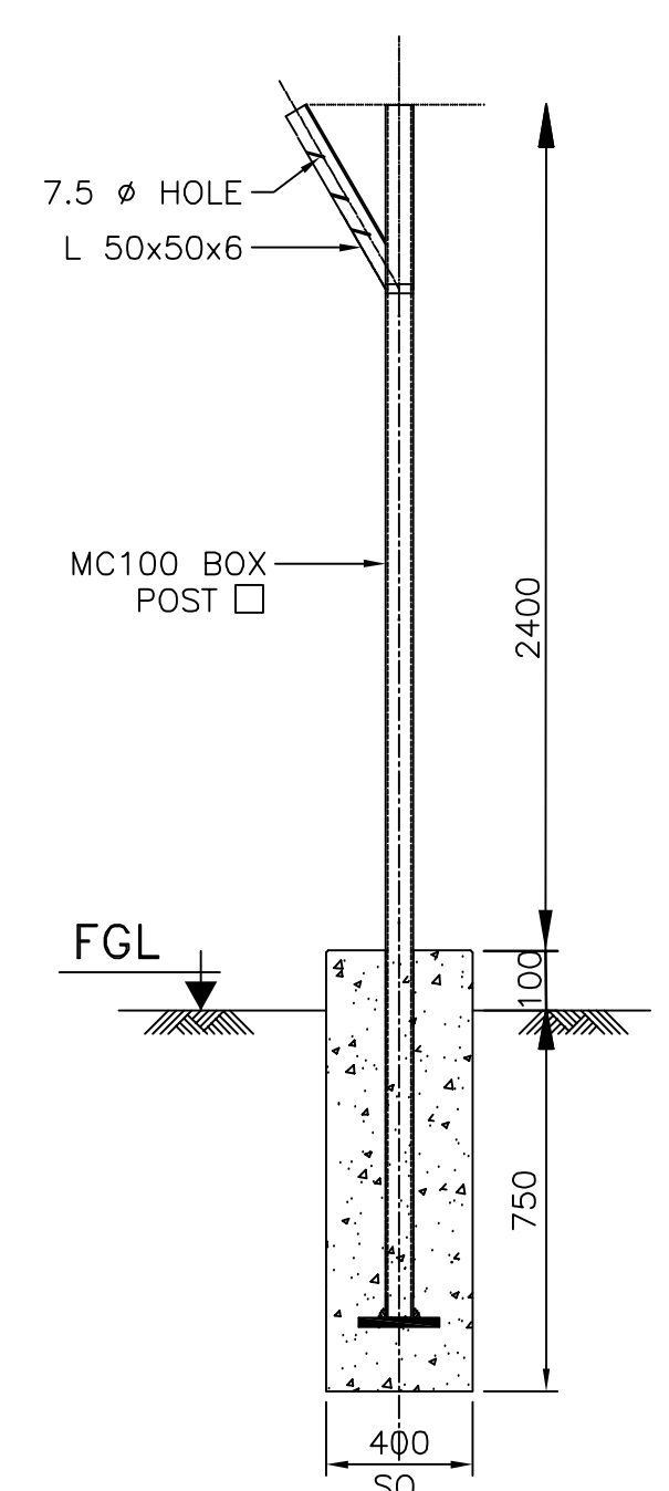
VIEW 1 (SCALE NTS) (DETAIL OF STEEL GATE POST)
