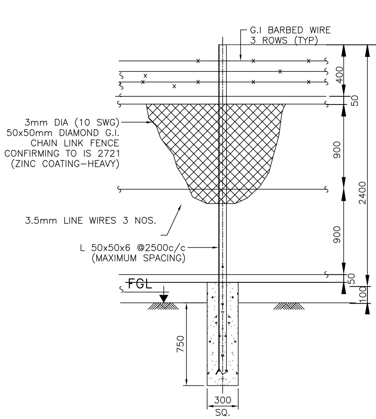
DETAIL OF INTERMEDIATE POST (SCALE NTS)
