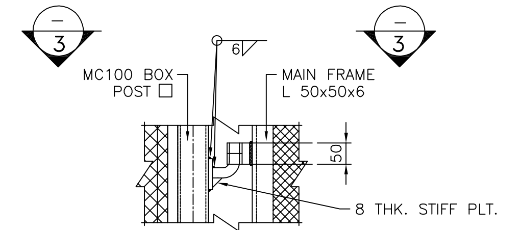
DETAIL B (SCALE NTS)
