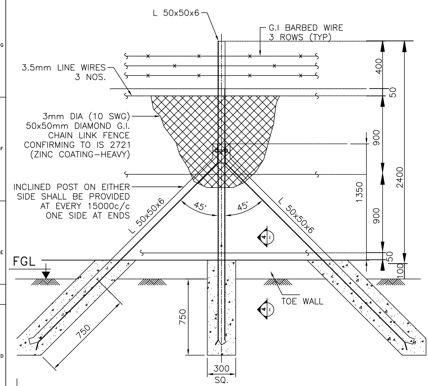
DETAIL OF STRAIN POST (SCALE NTS)
