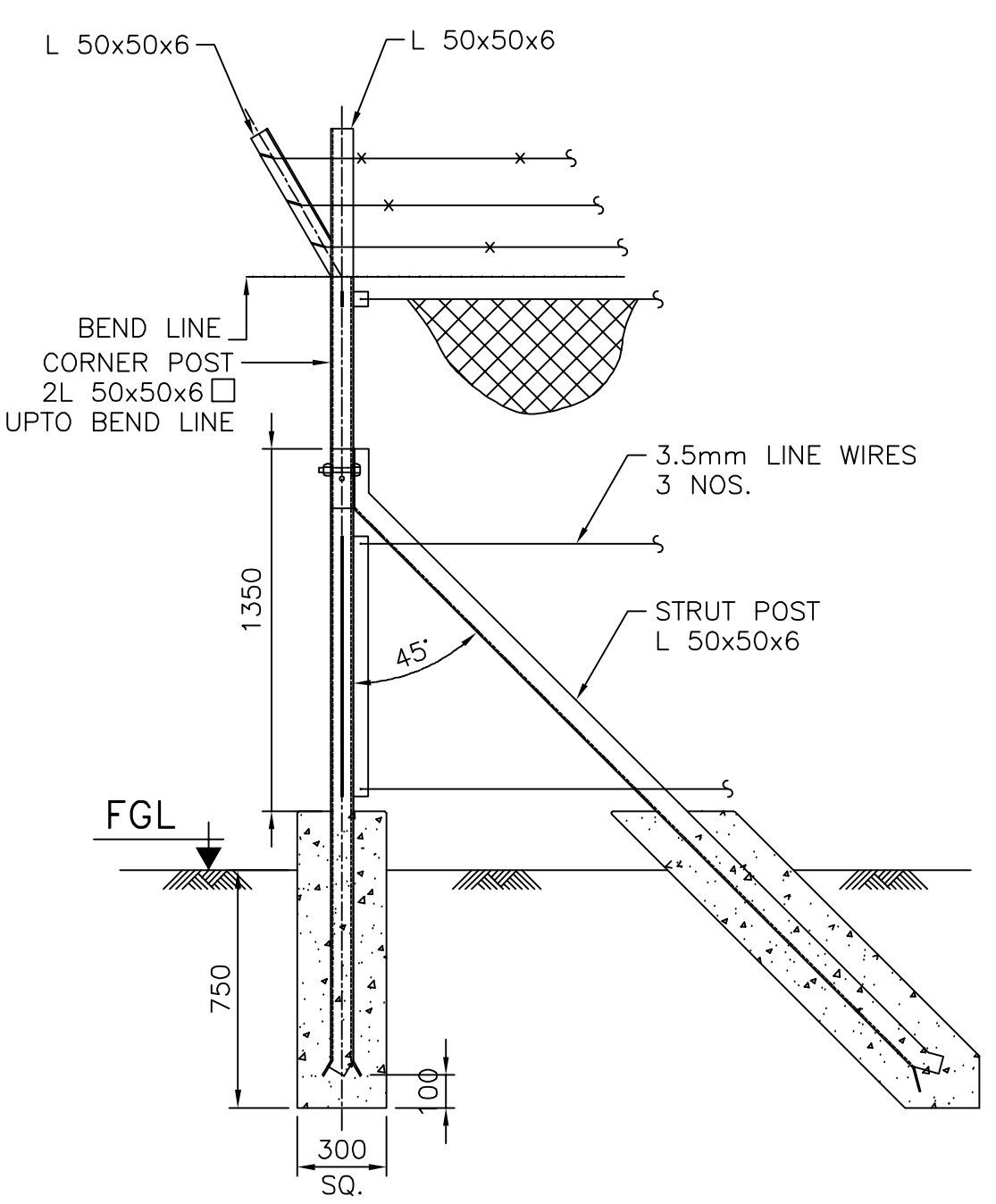
DETAIL OF CORNER POST (SCALE NTS)
