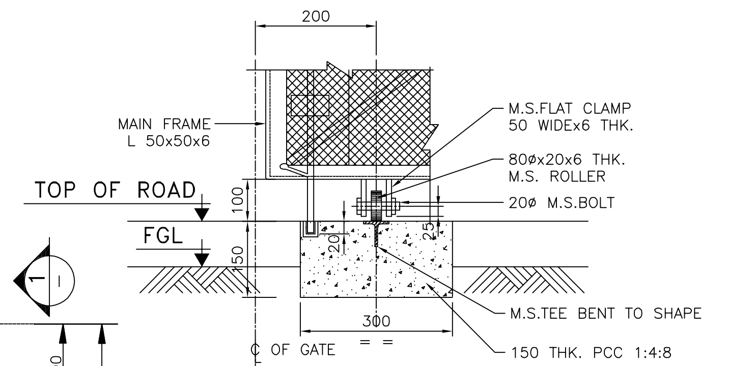
DETAIL A (SCALE NTS)
