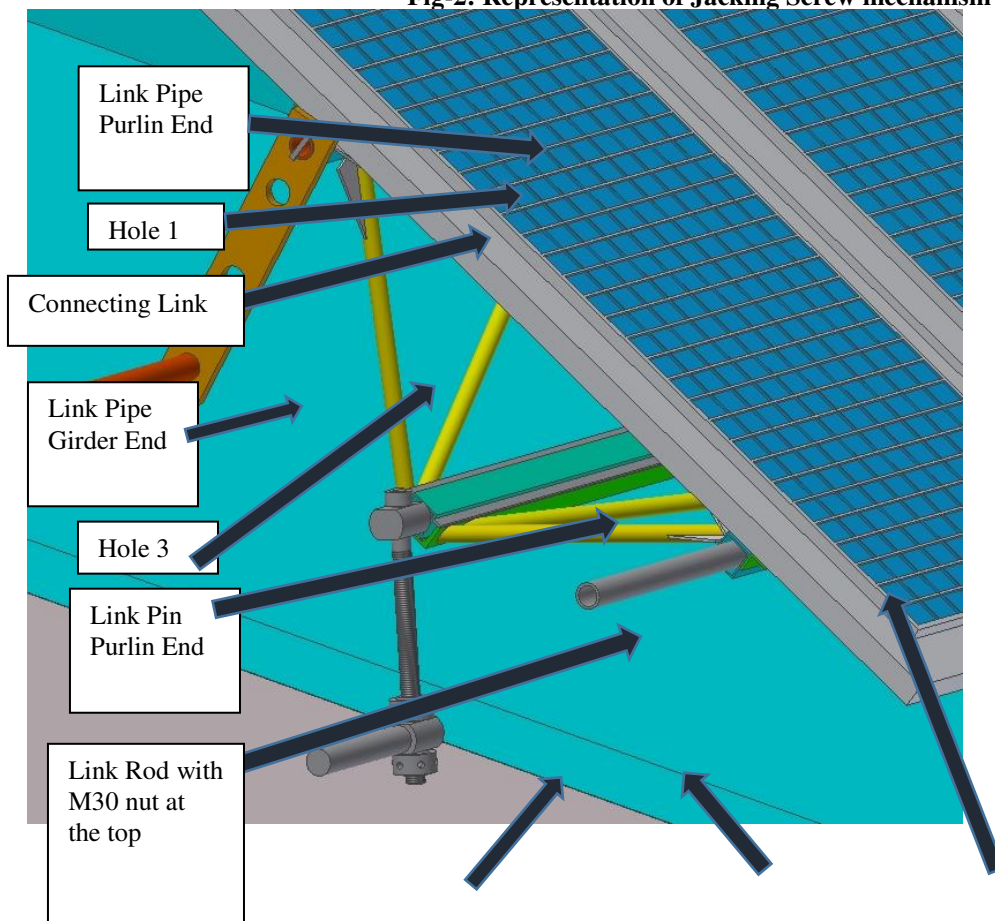
Fig-2: Representation of Jacking Screw mechanism
