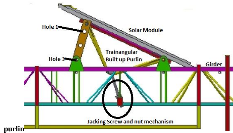
Fig-2: Representation of Jacking Screw mechanism
