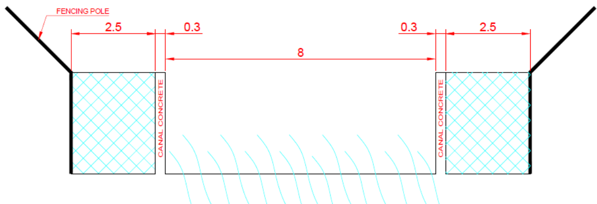
Fig-7: Cross Sectional View of the Canal at plant.
