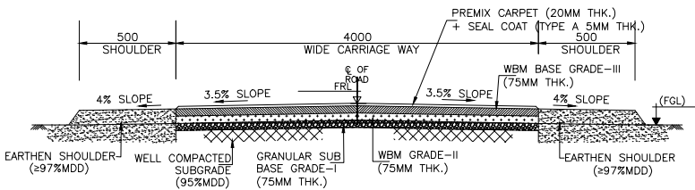
TYP. CROSS SECTION OF 4M WIDE APPROACH ROAD (As per IRC SP-20-VILLAGE/DIST ROAD DESIGN , FOR 45 VEHICLE/DAY WITH CBR 12.85%)
