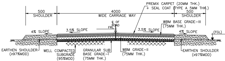
TYP. CROSS SECTION OF 4M WIDE PERIPHERAL ROAD (As per IRC SP-20-VILLAGE/DIST ROAD DESIGN , FOR 45 VEHICLE/DAY WITH CBR 12.85%)
