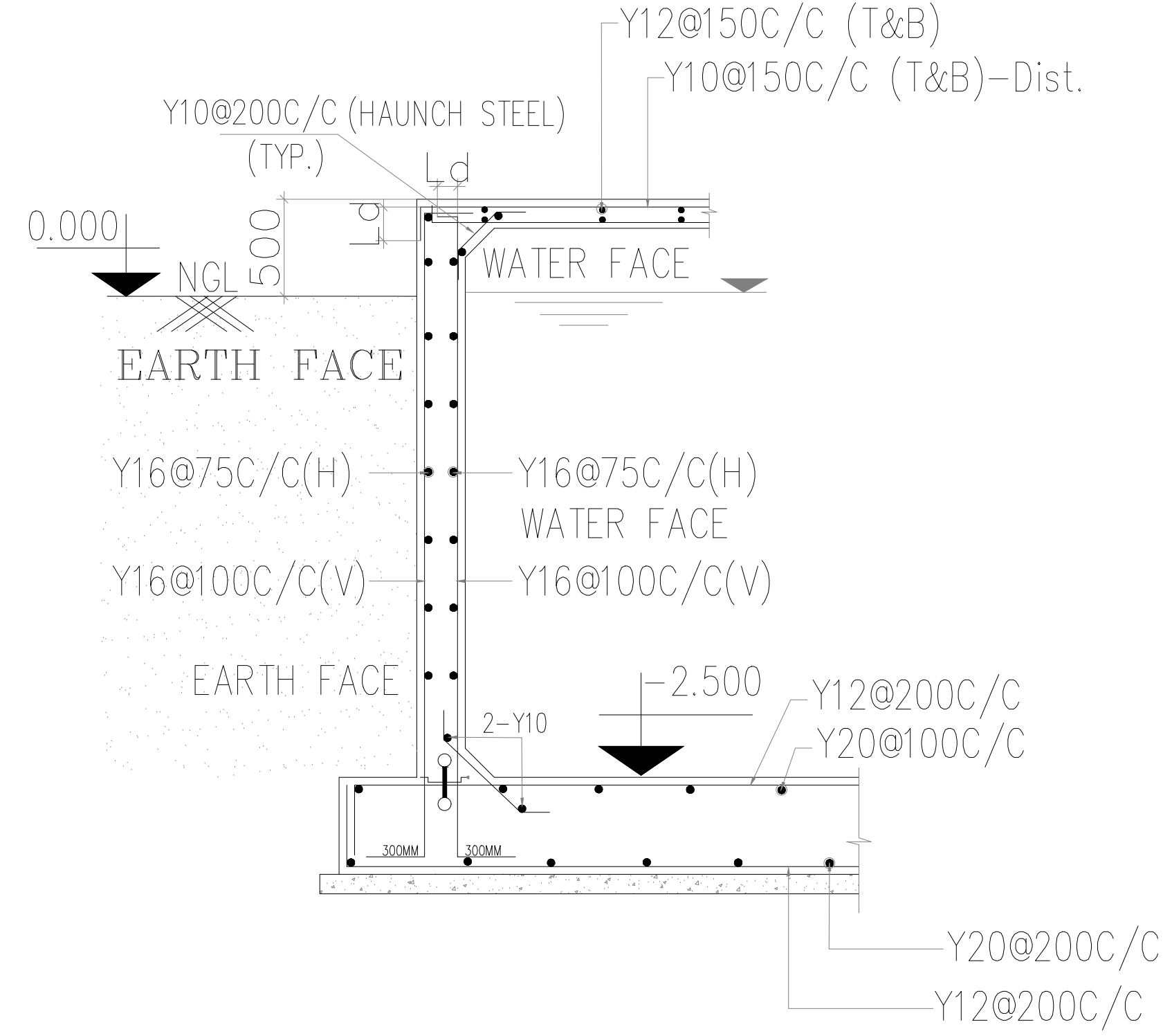
WALL-2 DETAIL SEC-DD REINFORCEMENT DETAIL
