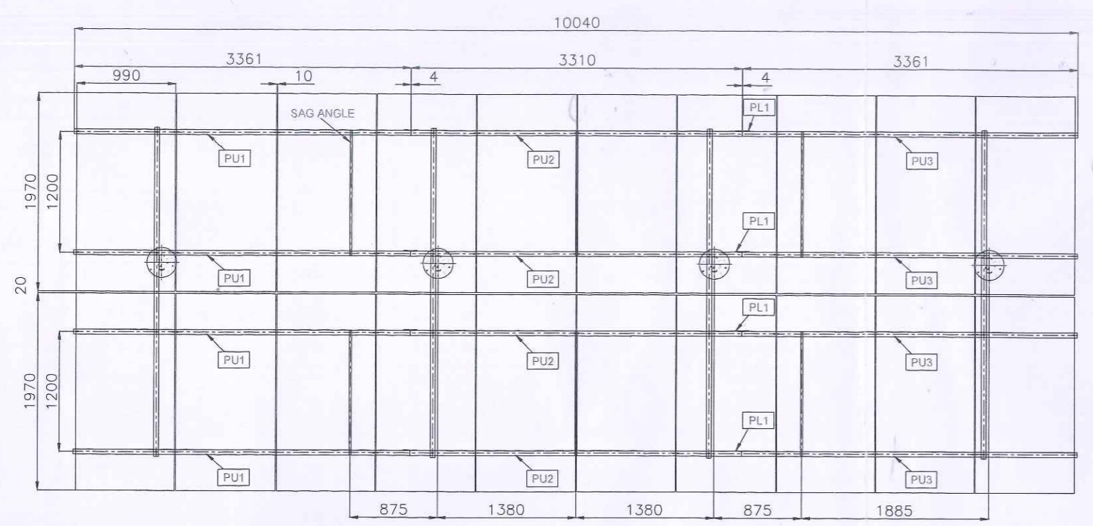
PLAN OF STRUCTURE (WITH SOLAR MODULE) FOR 0°
