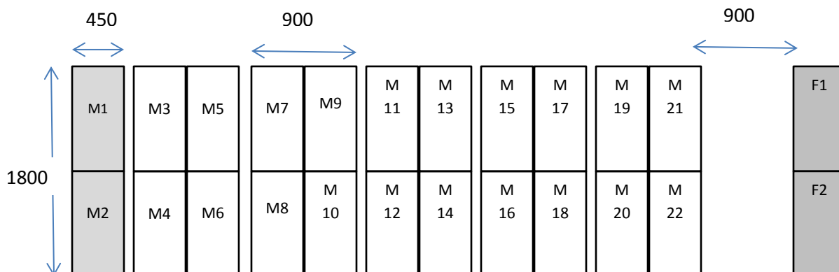
Fig 2: Overall layout
