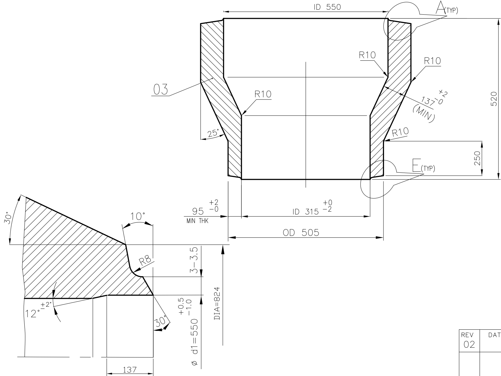
DETAIL-A
