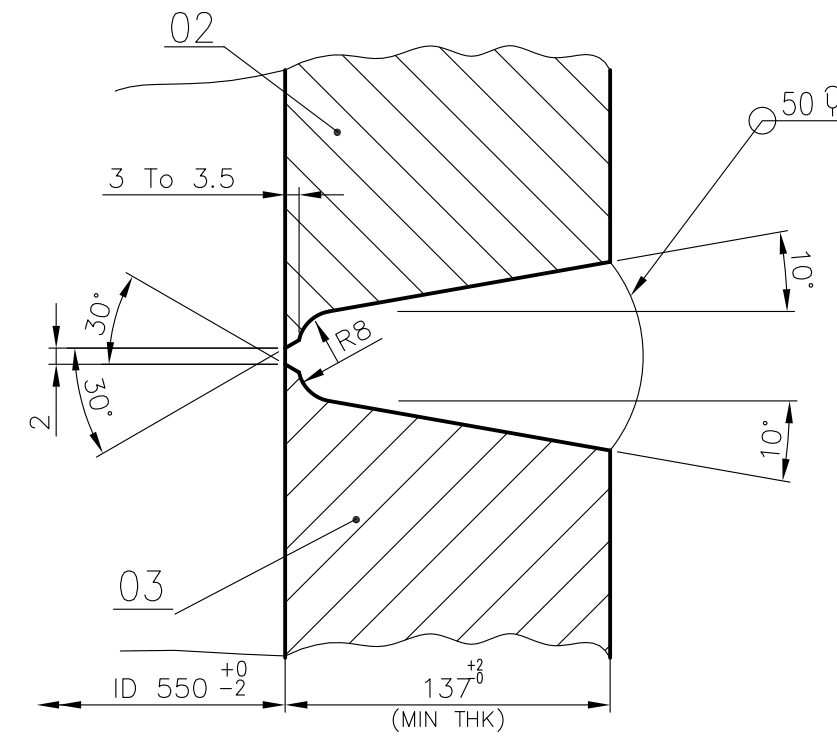
DETAIL-C
