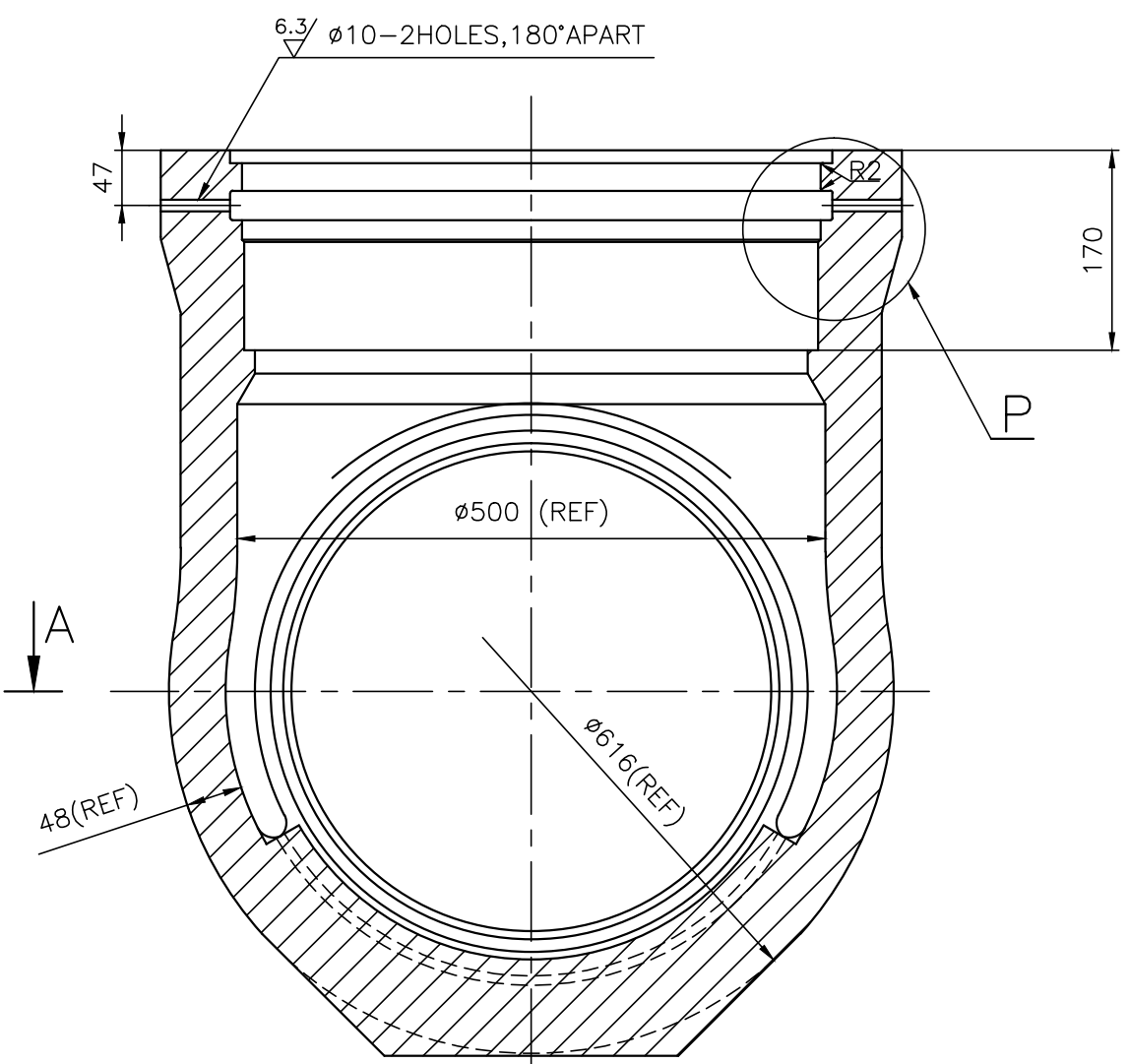
SECTION-BB
