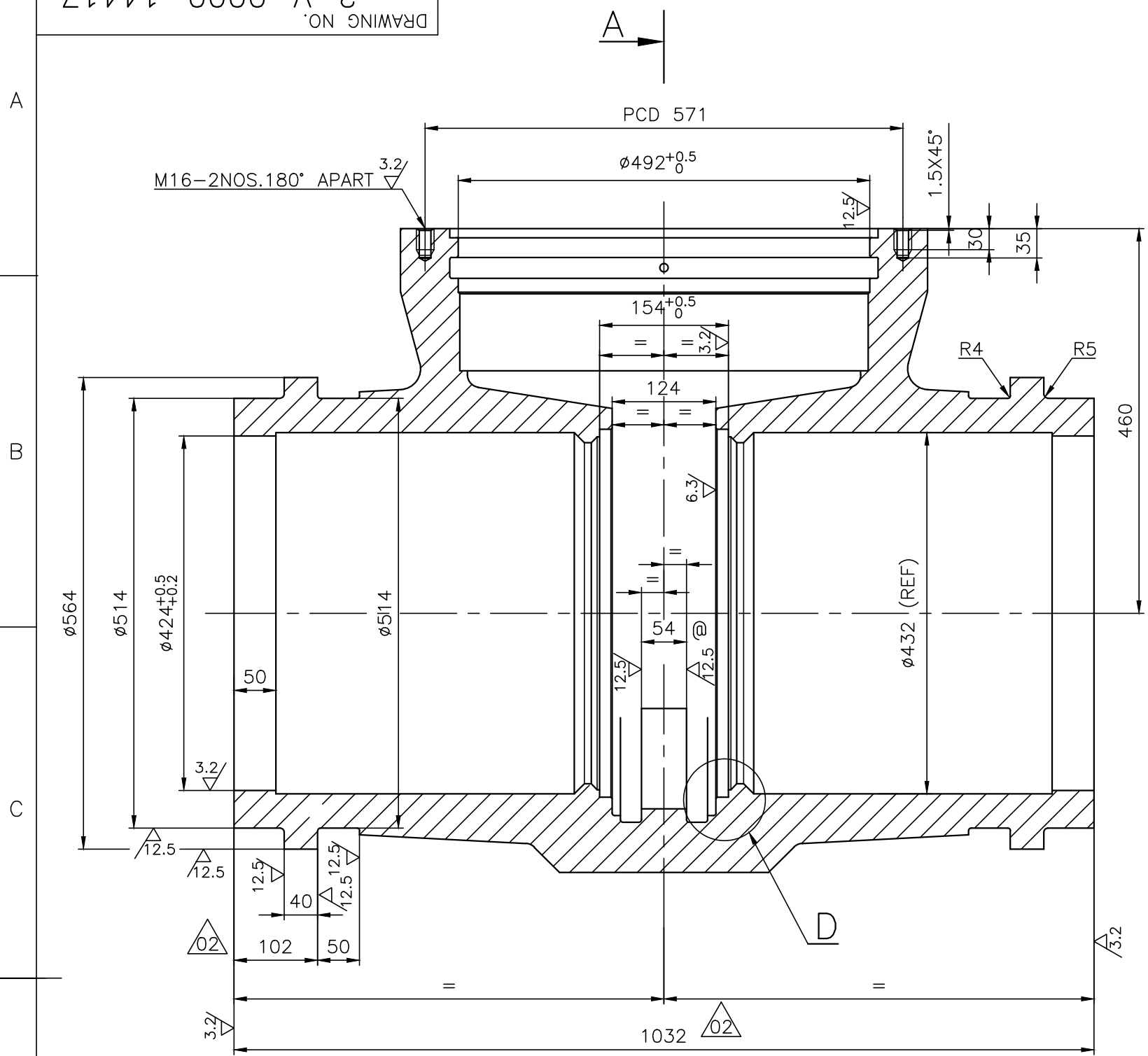
SECTION-CC
