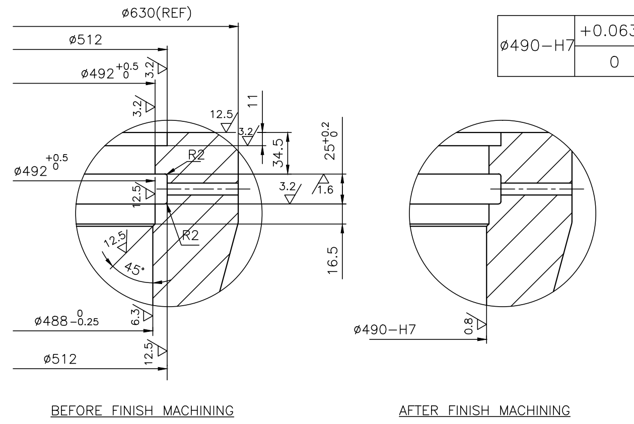
DETAIL-P
