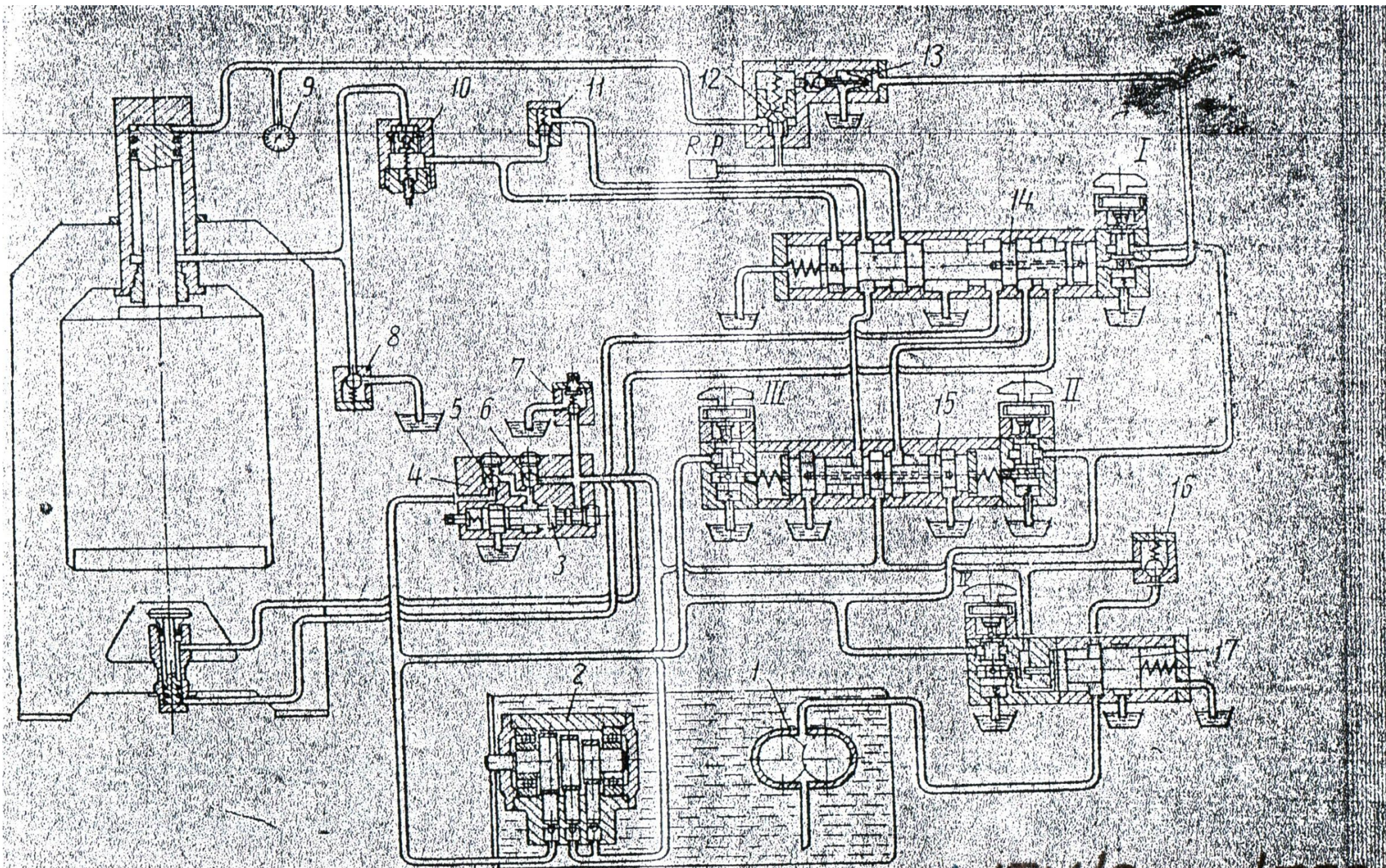
Fig. 14 Hydraulic Circuit
