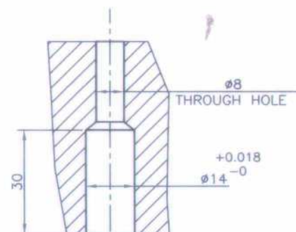
HOLE DETAIL-P
