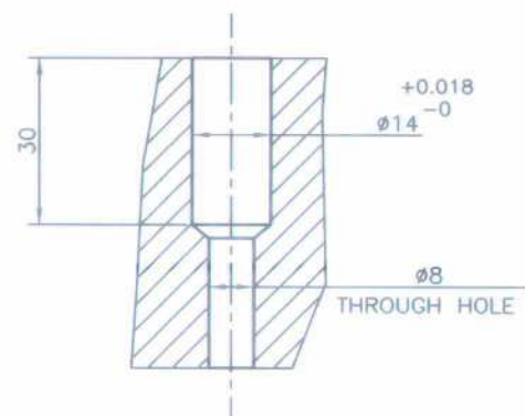
HOLE DETAIL-P
