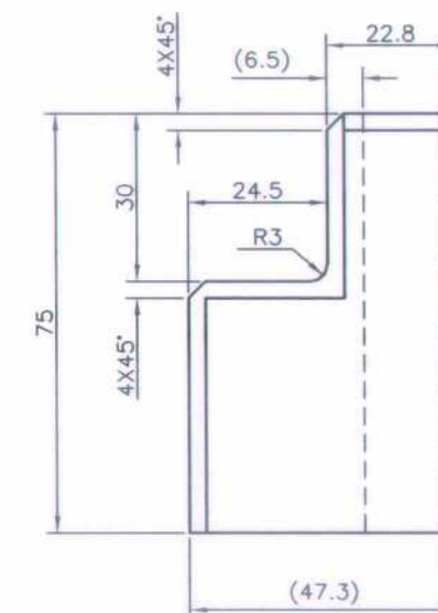
202 FIXED JAW
