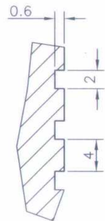
SERRATION DETAILS-K
