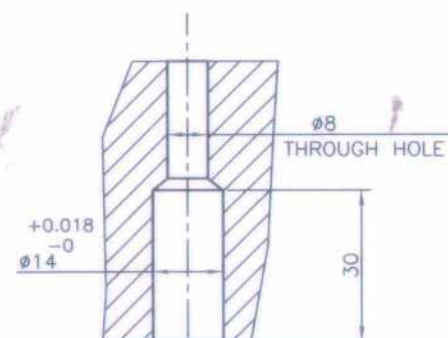
HOLE DETAIL-P
