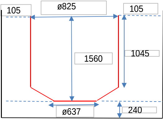
5T Furnace Former Dimesions
