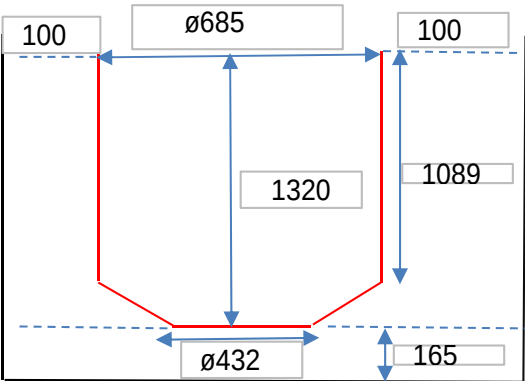
2.5T Furnace Former Dimesions
