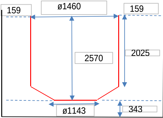
20T Furnace Former Dimesions
