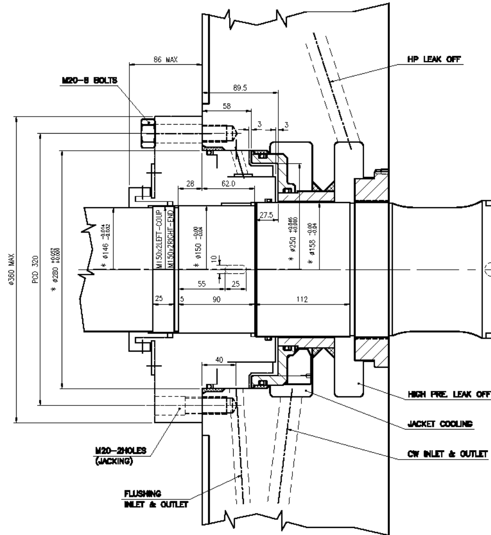
COORDINATION DIAGRAM FOR SHAFT SEAL, MDG405 BFP
