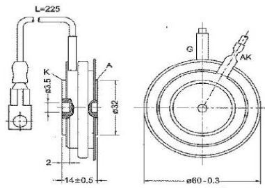
OUTLINE DIAGRAM-13
