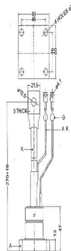
OUTLINE DIAGRAM-12
