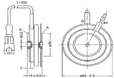
OUTLINE DIAGRAM-14
