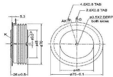
OUTLINE DIAGRAM-14
