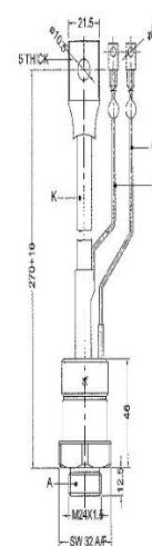
OUTLINE DIAGRAM-11
