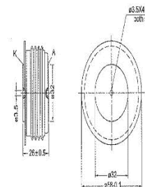
OUTLINE DIAGRAM-8
