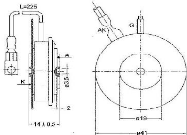
OUTLINE DIAGRAM-13
