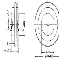
OUTLINE DIAGRAM-6
