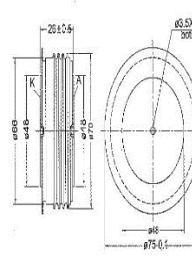
OUTLINE DIAGRAM-9
