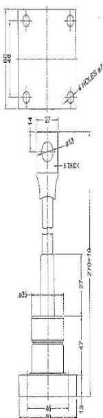
OUTLINE DIAGRAM-4
