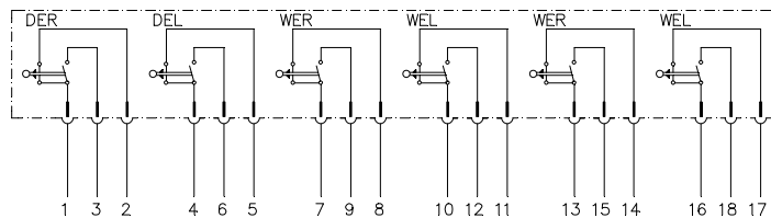
WIRING DIAGRAM
