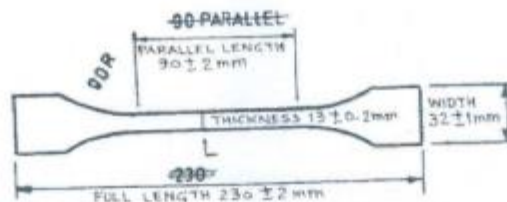
Fig. 1 Specimen for Tensile Strength Test.
