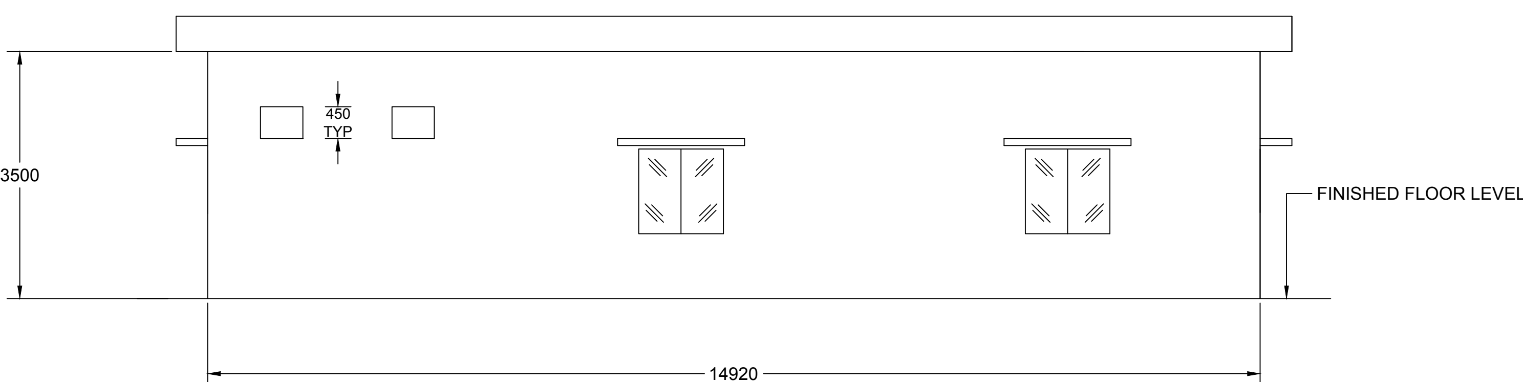
SOUTH ELEVATION
