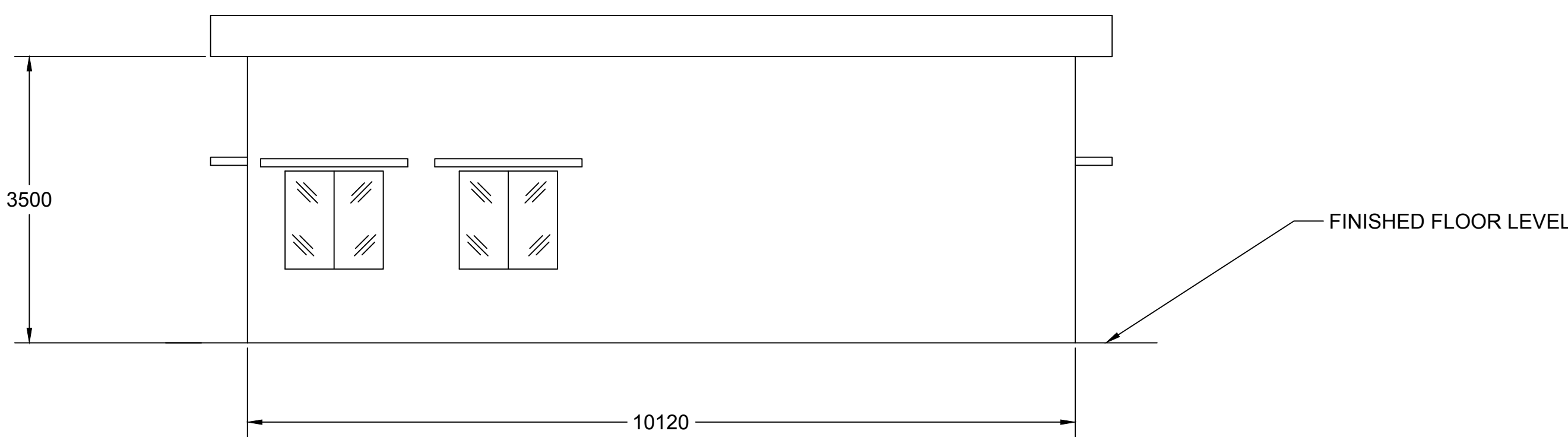
WEST ELEVATION
