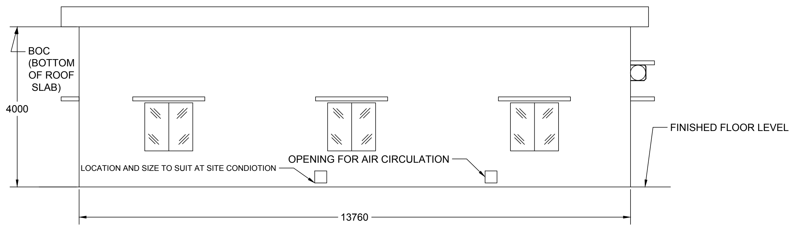
NORTH ELEVATION
