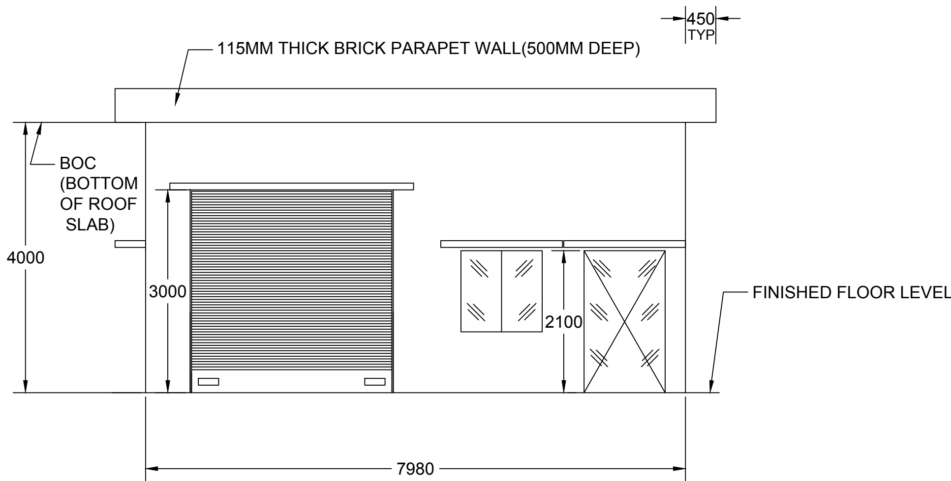
WEST ELEVATION
