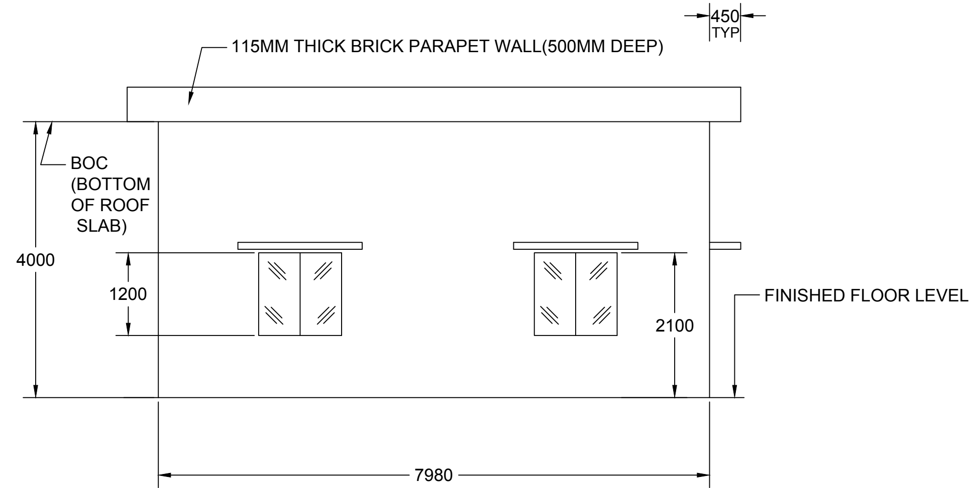
EAST ELEVATION
