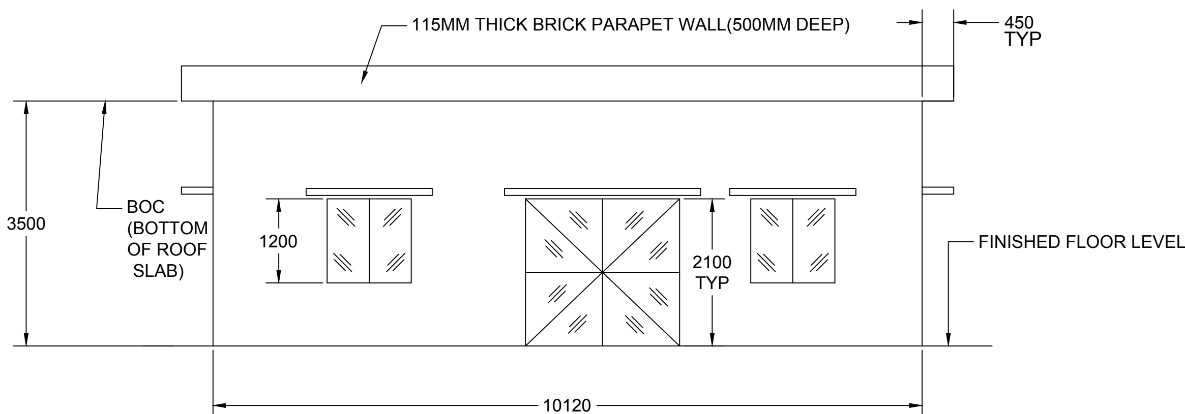
EAST ELEVATION
