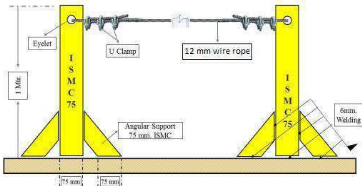
Fig. 13.2.1.1 Lifeline Post
