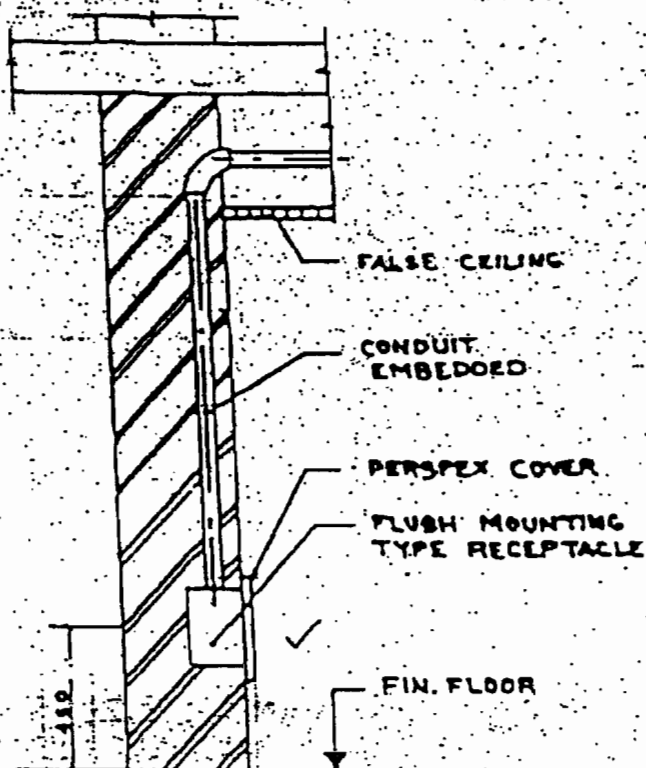
RECEPTACLE - TYPE 'R' (WALL MOUNTING)
