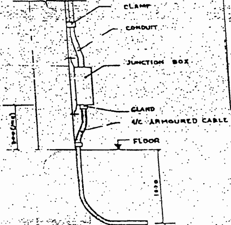
JUNCTION BOX MOUNTING (TYP)
