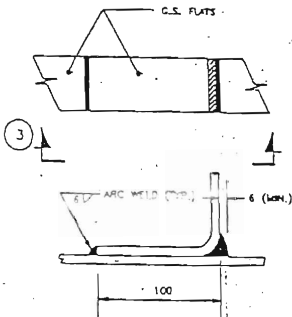
SECTION - ③
