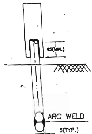
SECTION 3-3
