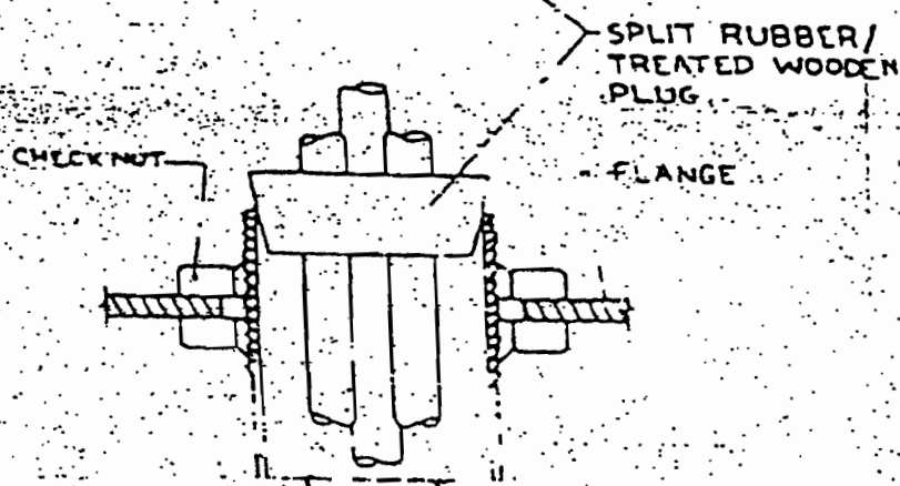
CLAMPING OF WIRES IN CONDUIT VERTICAL RUN
