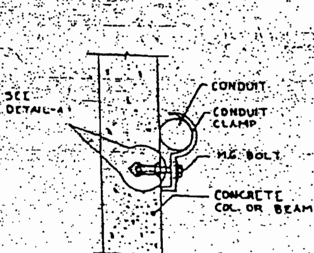
SINGLE CONDUIT RUN ON CONCRETE SURFACE
