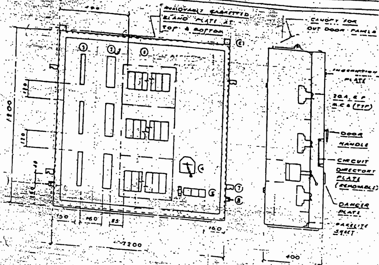
FRONT VIEW (DOOR REMOVED)
