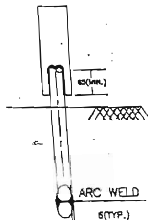
SECTION 3-3
