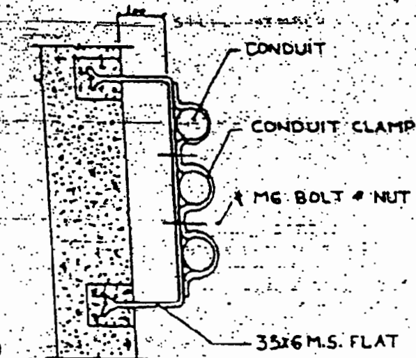
GROUP OF CONDUITS RUN ON CONCRETE SURFACE
