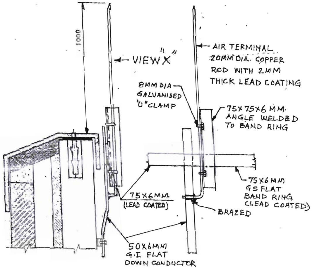
SECTION 2-2
