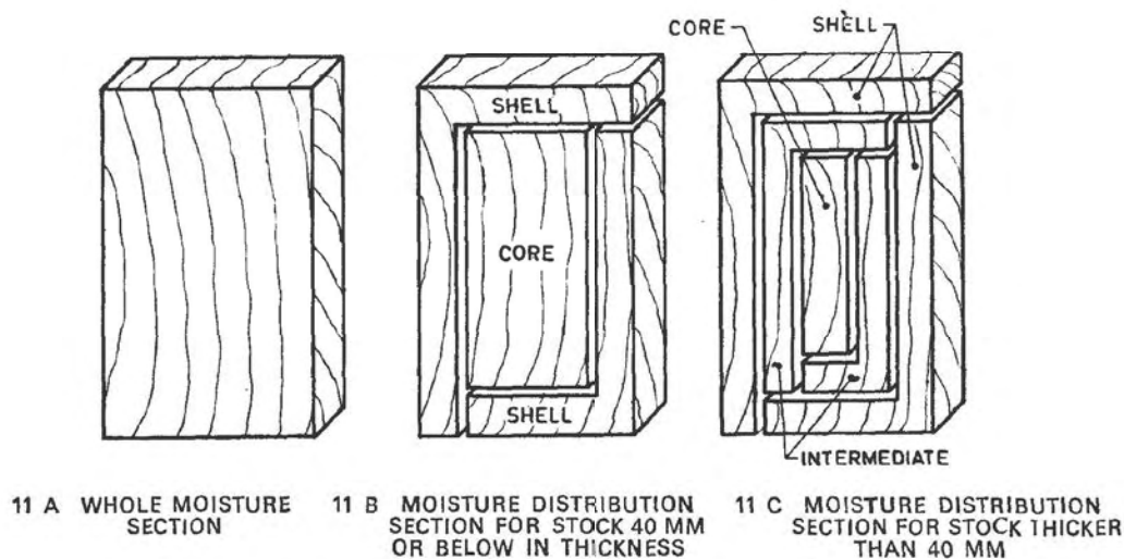
FIG. 11 FINAL MOISTURE SECTIONS
