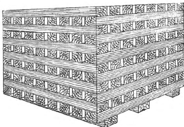
FIG. 3 OPEN CRIB STACKING
