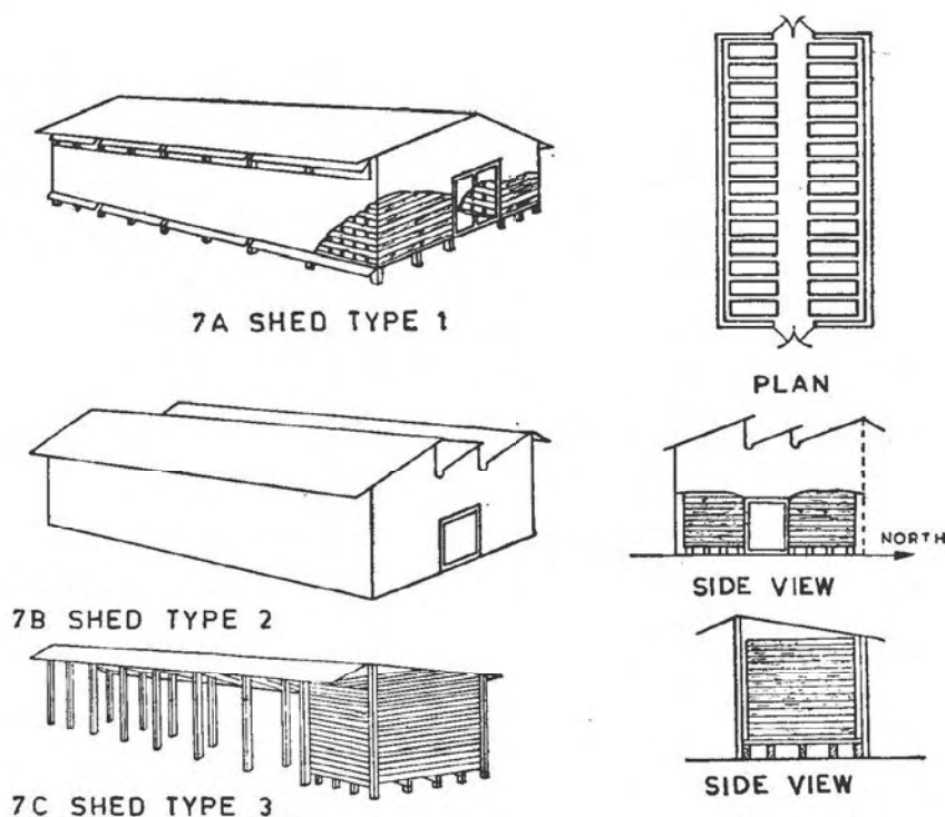
FIG. 7 AIR SEASONING SHEDS
