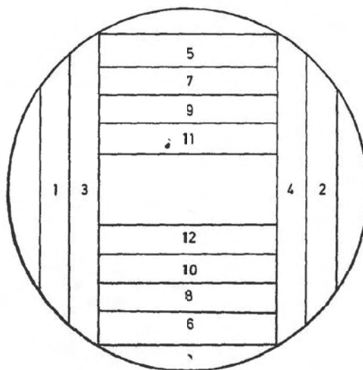
FIG. 8 BALANCED TANGENTIAL SAWING
