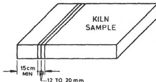
FIG. 10 TEST SECTIONS FOR FINAL CHECK
