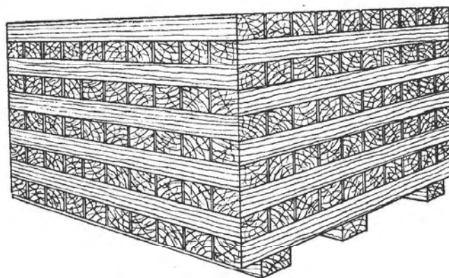
FIG. 2 CLOSE CRIB STACKING
