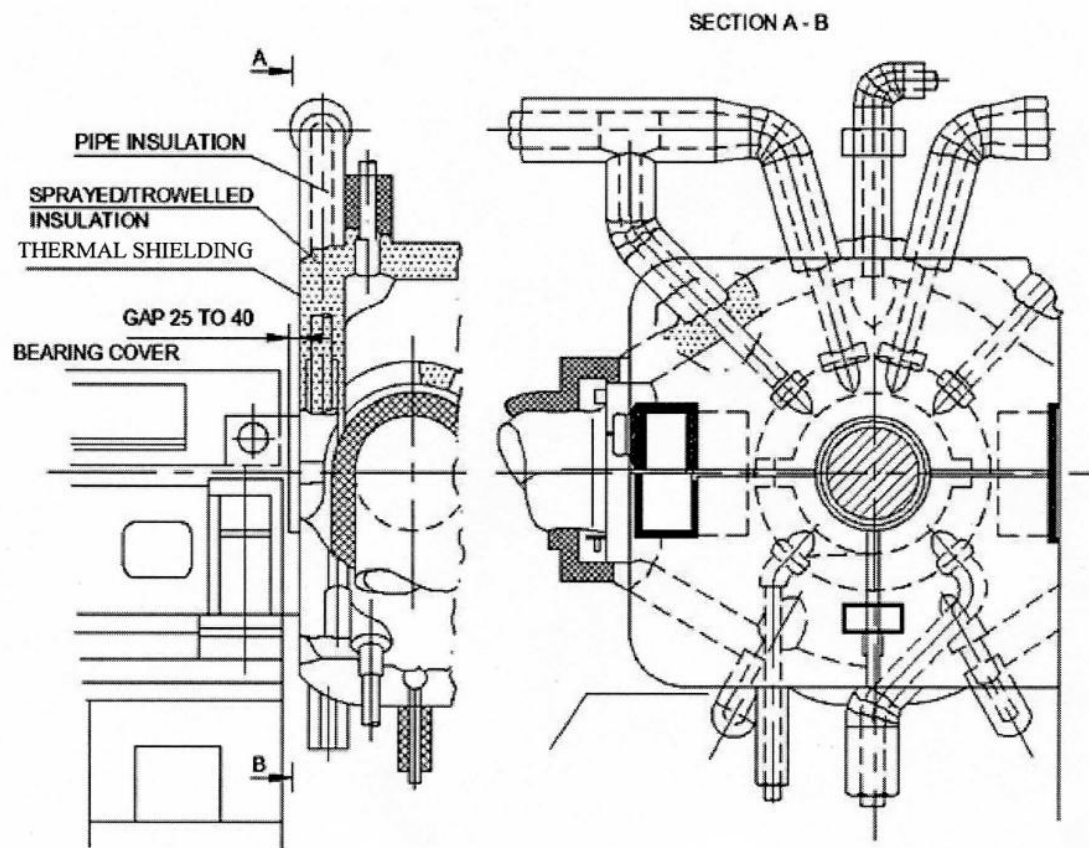
Figure-1: Arrangement Of Thermal Shielding
