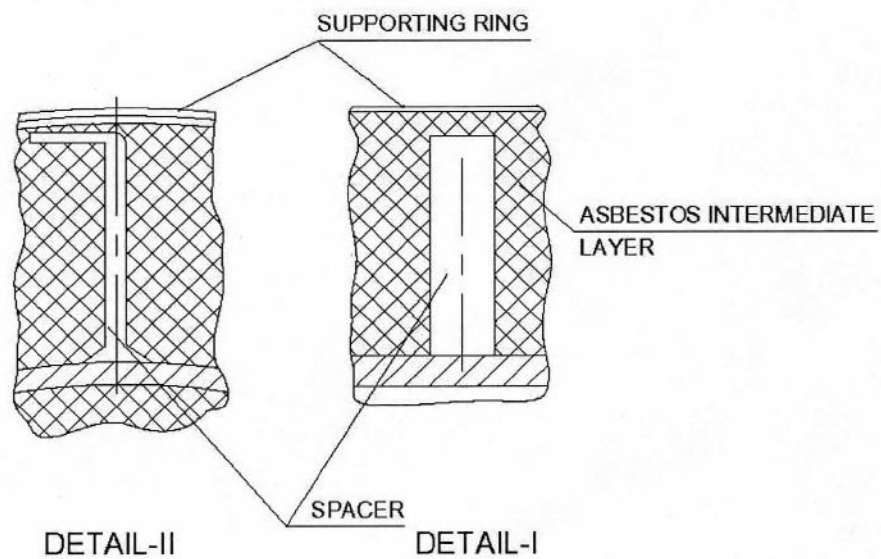
FIG.-5 STANDARD PIPE INSULATION
