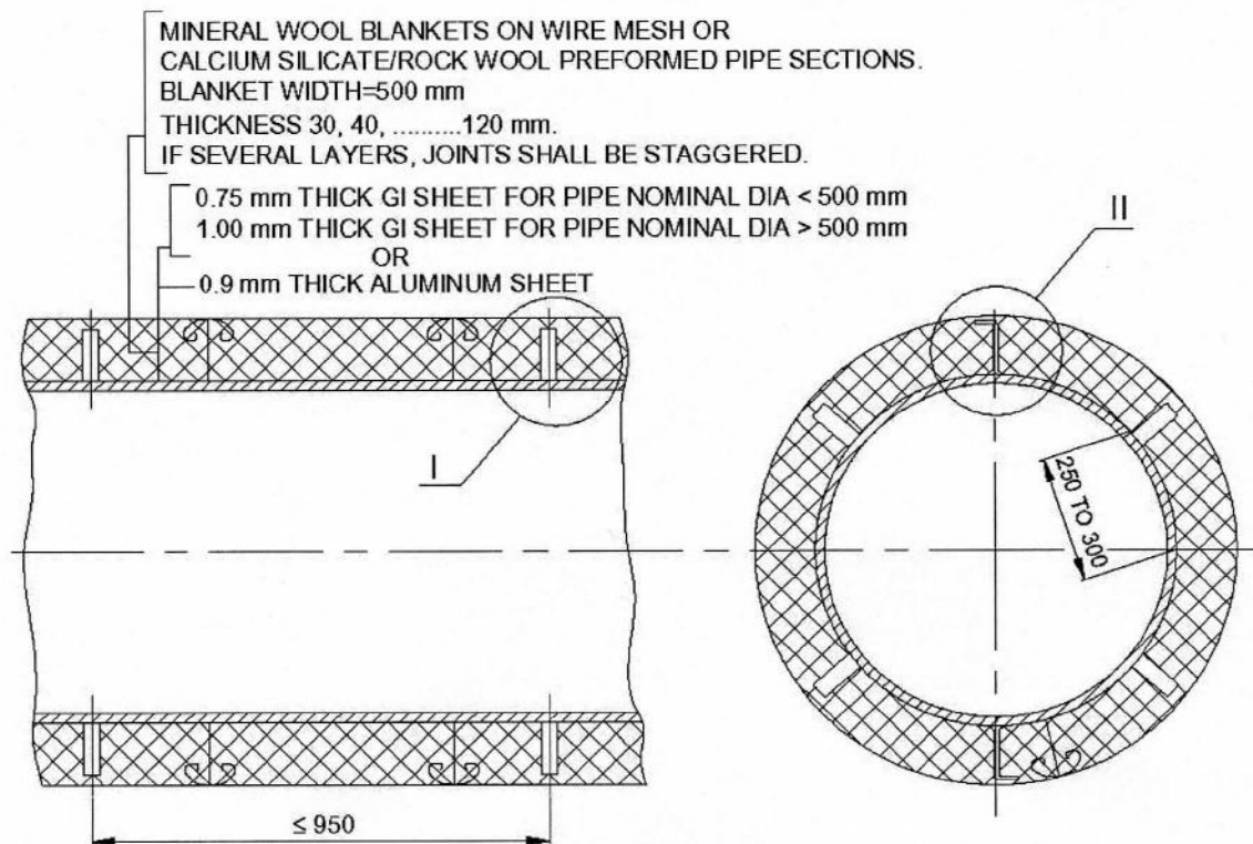
FIG.-5 STANDARD PIPE INSULATION
