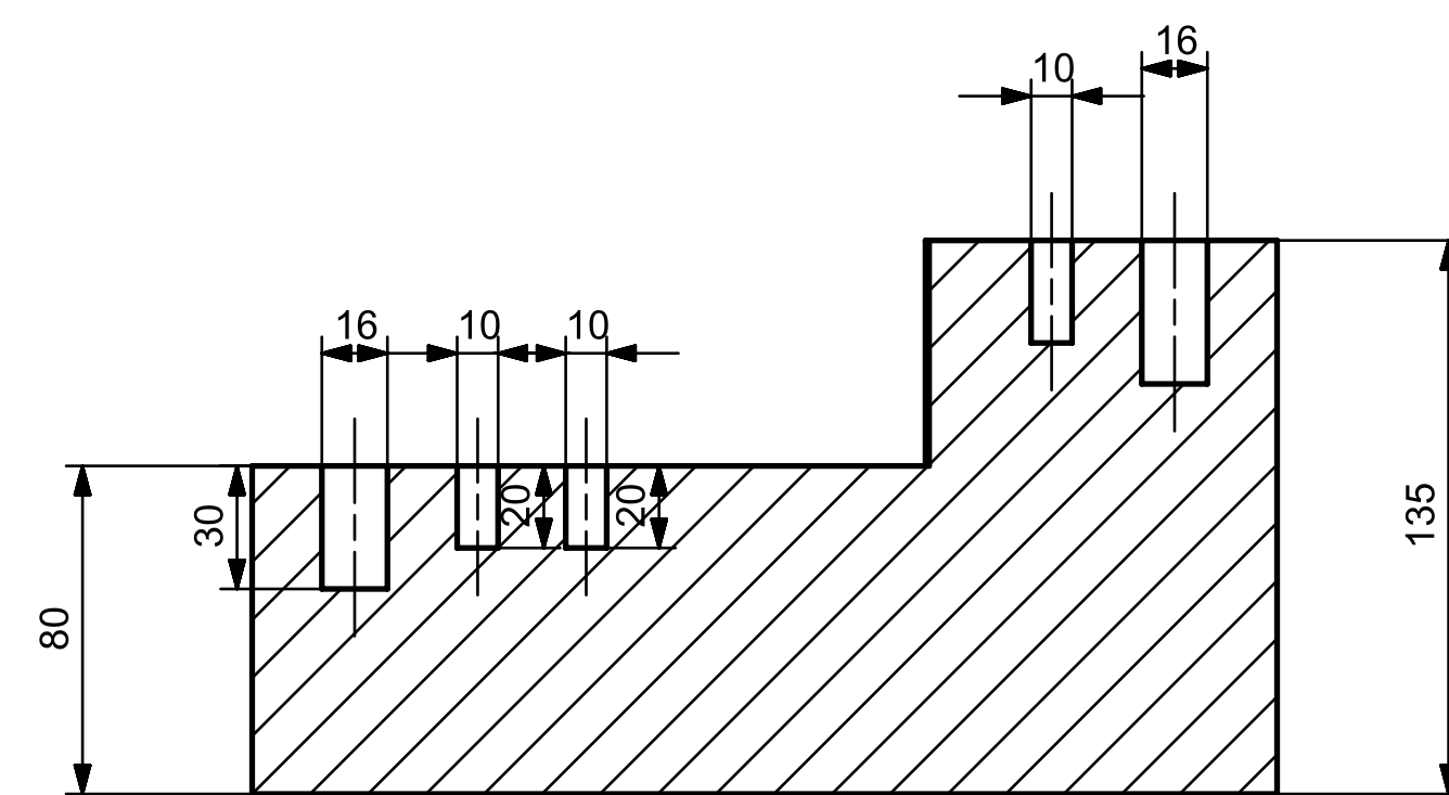
SECTION C-C
