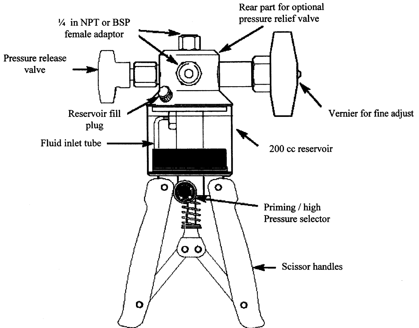
Representative diagram of the Hydraulic Hand Pump Required
