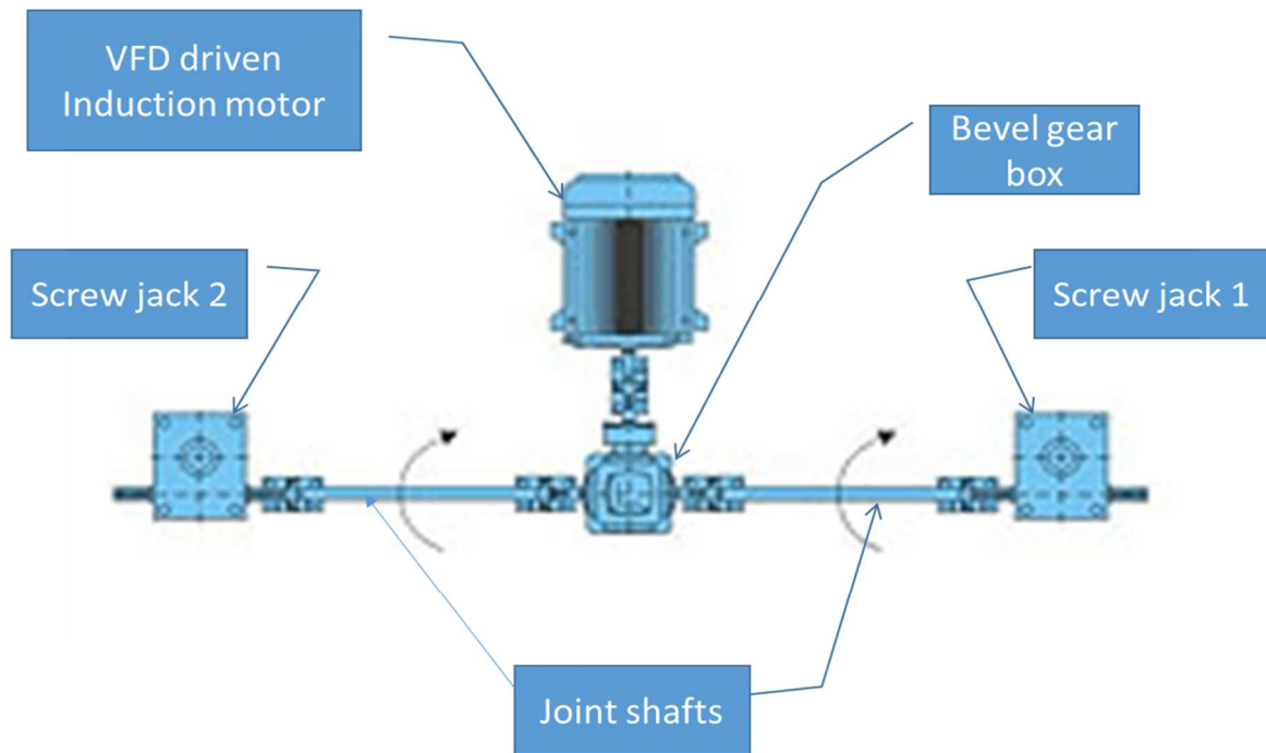
Figure 2. Block diagram for the intended retrofit mechanism (Top View)
