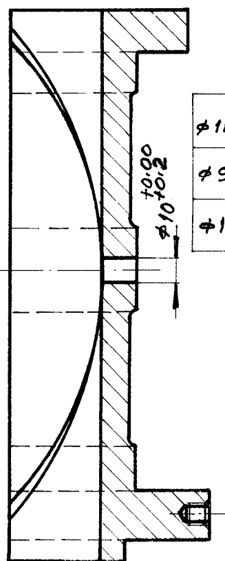
DETAIL P-P
