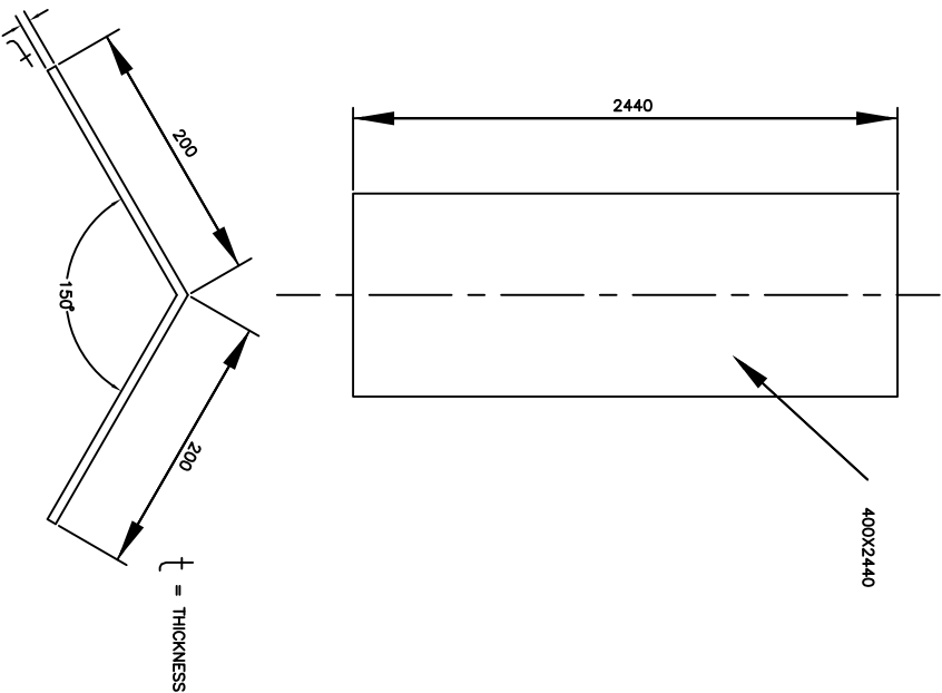
DETAILS OF RIDGE PIECE
