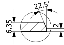
DETAIL D SCALE 1:1
