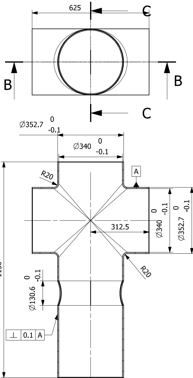
SECTION B-B
