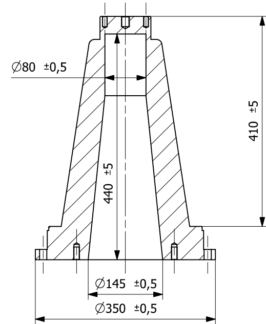
SECTION C-C
