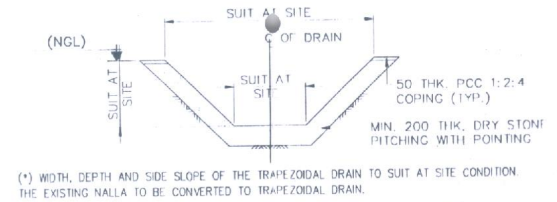
TYP. DETAIL OF TRAPEZOIDAL DRAIN ND1 (SCALE 1:50)
