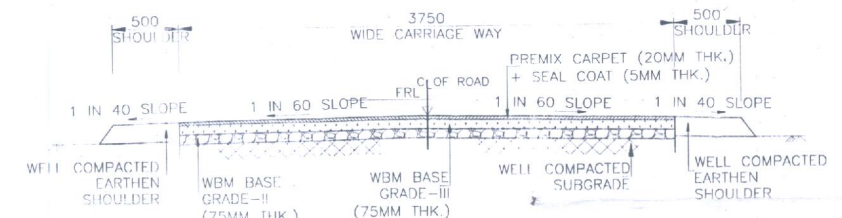
TYP. CROSS SECTION OF 3.75M CARRIAGEWAY BITUMEN ROAD (SCALE 1:25)
