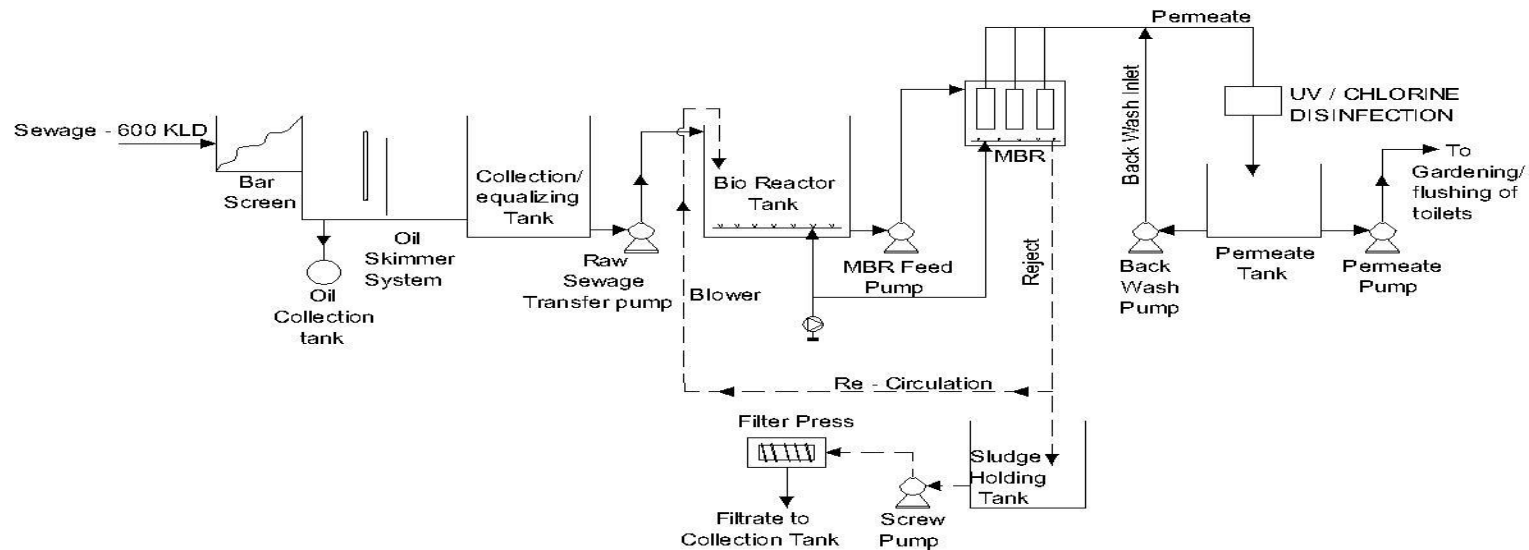
Indicative Process Flow Diagram
