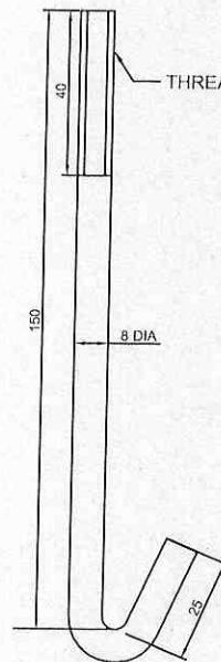
ITEM-003 J-HOOK SIZE=8mm DIAx150LONGx25mm. SUITABLE FOR FIXING ON ANGLE 75x75x6mm
