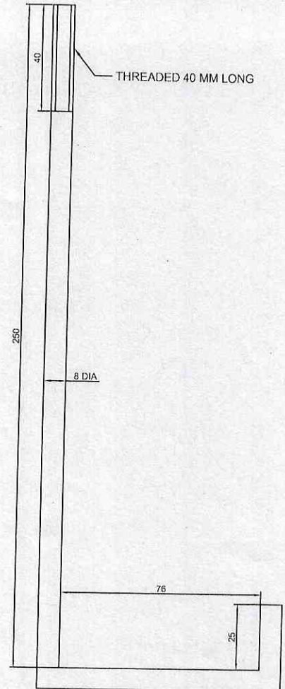
ITEM-005 L-HOOK SIZE=8mm DIAx250LONGx76mmx25mm. SUITABLE FOR FIXING ON CHANNEL 150mmx75mm
