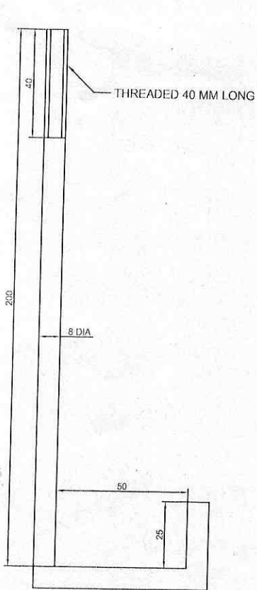
ITEM-007 L-HOOK SIZE=8mm DIAx200LONGx50mmx25mm. SUITABLE FOR FIXING ON CHANNEL 100mmx50mm
