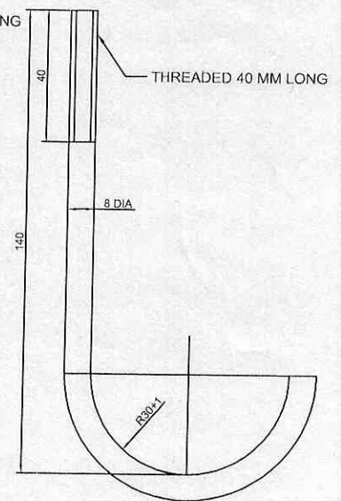
ITEM-004 J-HOOK SIZE=8mm DIAx140LONGx25mm. SUITABLE FOR FIXING ON 50NB PIPE
