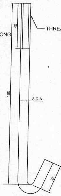
ITEM-002 J-HOOK SIZE=8mm DIAx160LONGx25mm. SUITABLE FOR FIXING ON ANGLE 65x65x6mm
