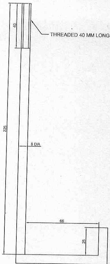
ITEM-006 L-HOOK SIZE=8mm DIAx225LONGx66mmx25mm. SUITABLE FOR FIXING ON CHANNEL 125mmx65mm
