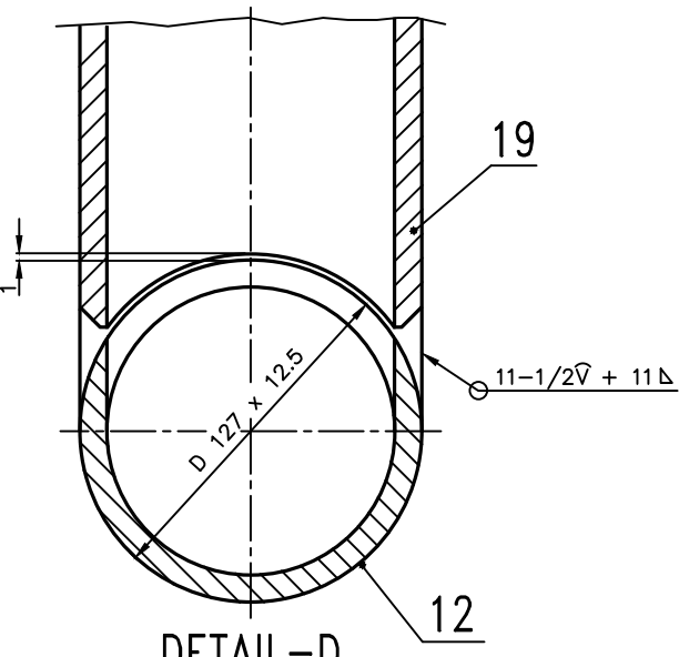
DETAIL-D WELDING DETAIL OF ITEM No 19 WITH 12
