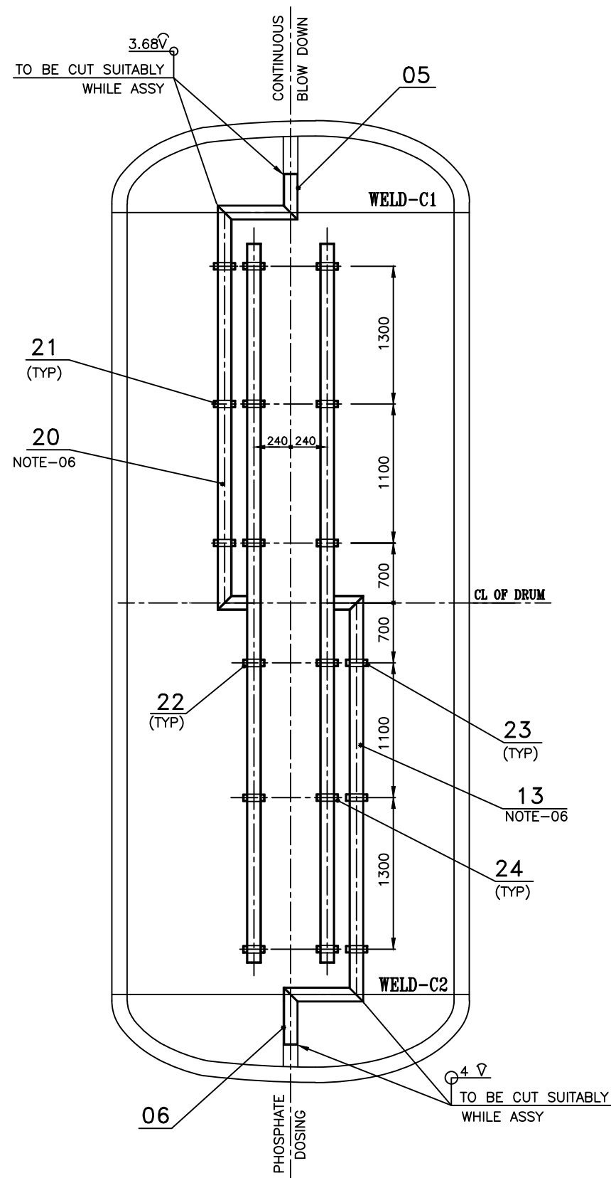
SECTION-CC (DETAIL OF PHOSPHATING & CBD PIPINGS)
