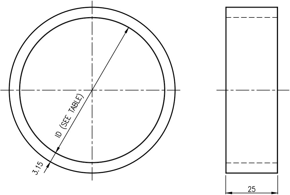
DETAIL OF ITEM NO. 01 & 02
