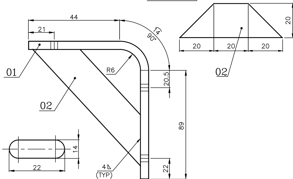
DETAIL-A
