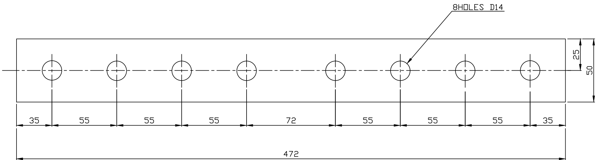
DEVELOPED VIEW OF ITEM No.02
