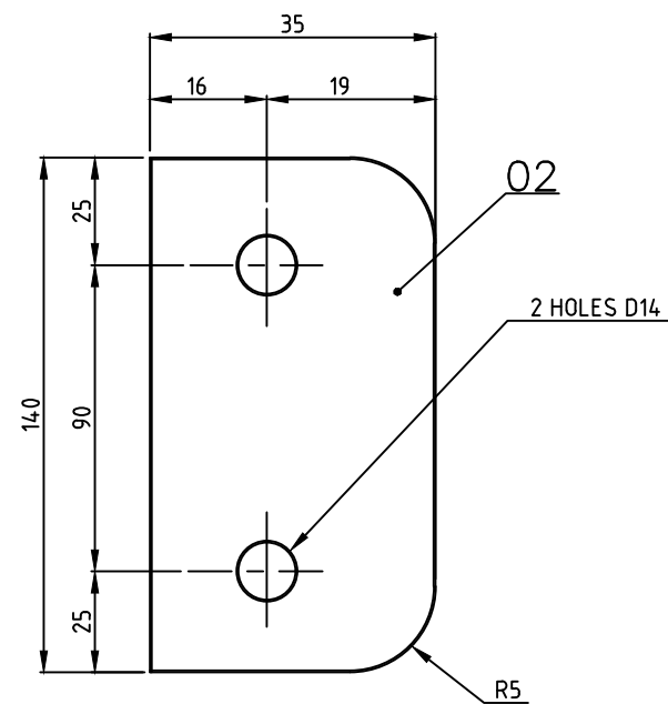
DETAILS OF ITEM No.02
