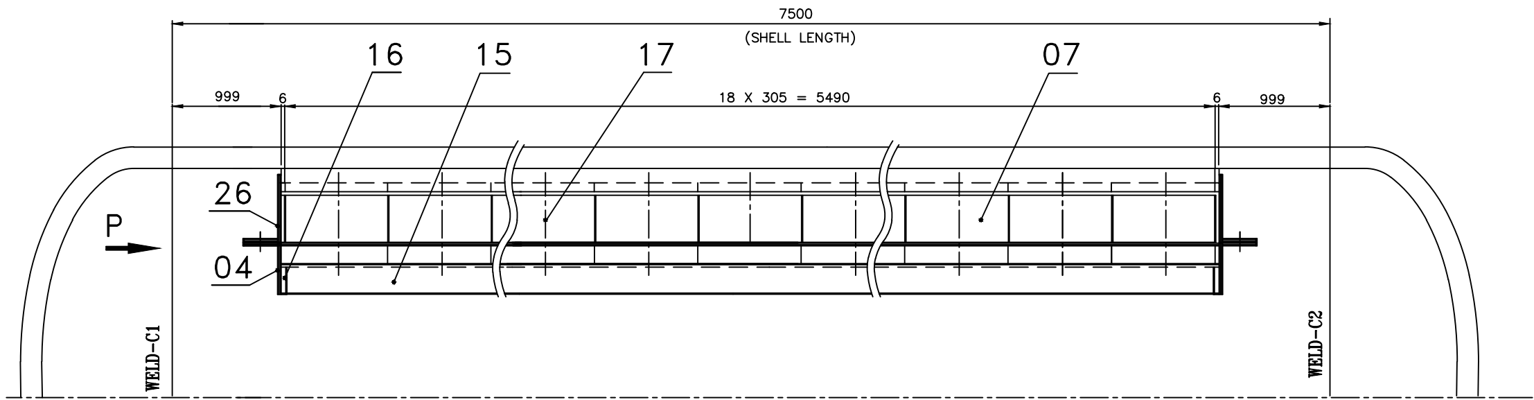
VIEW-Q
